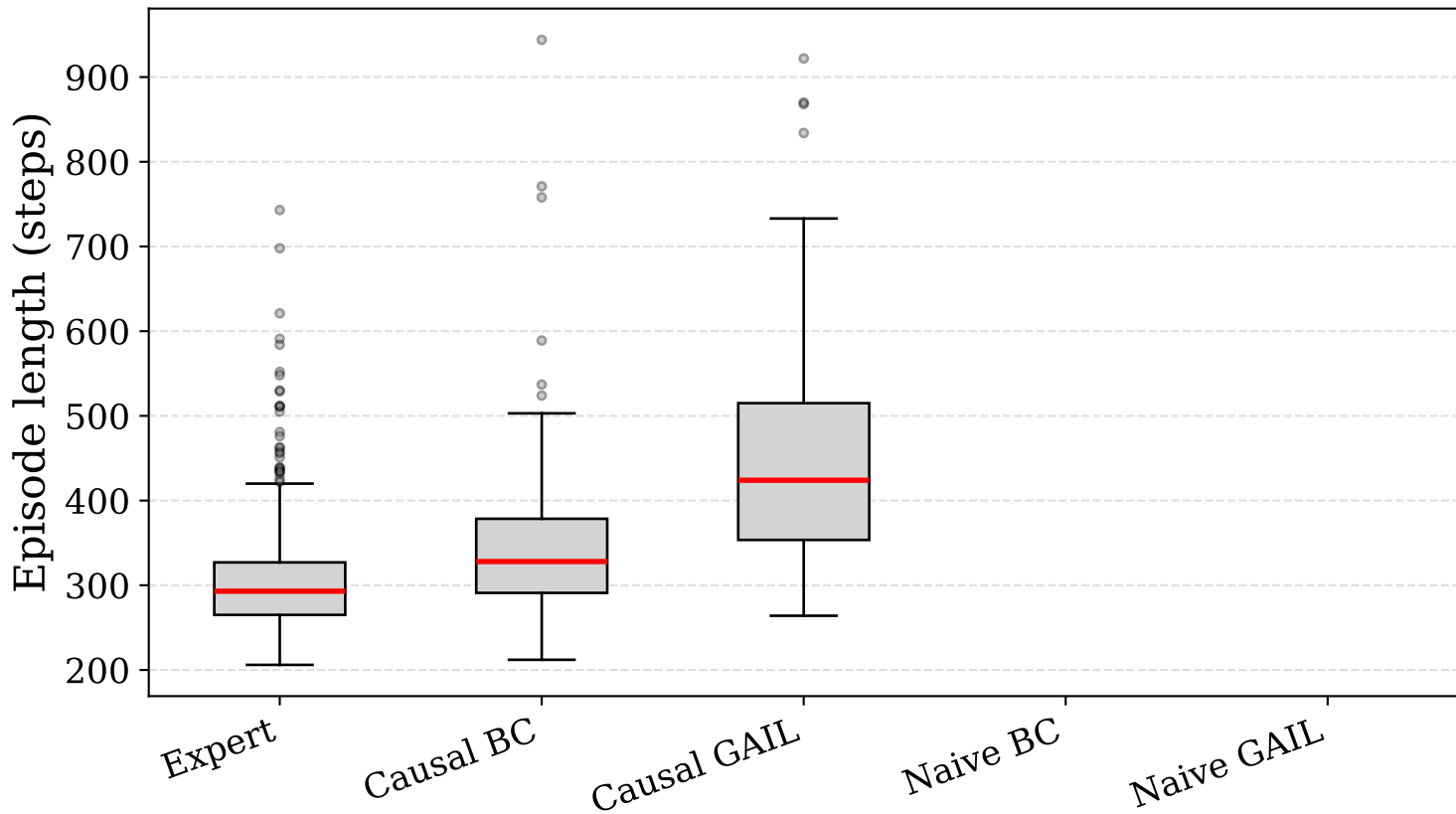
Ant Maze: Successful Episode Lengths (< 1000 steps)
