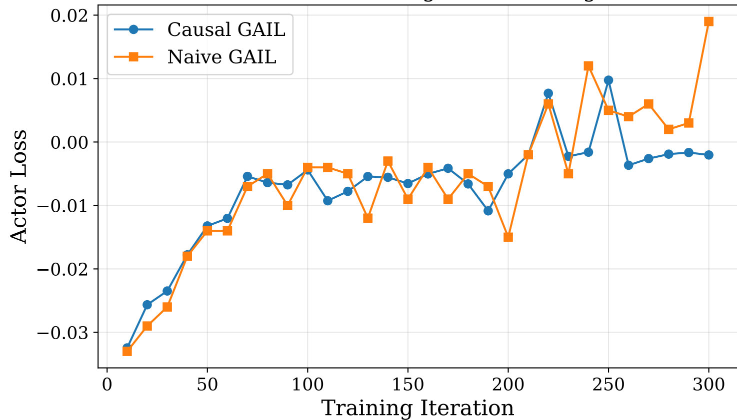
Actor Loss During GAIL Training
