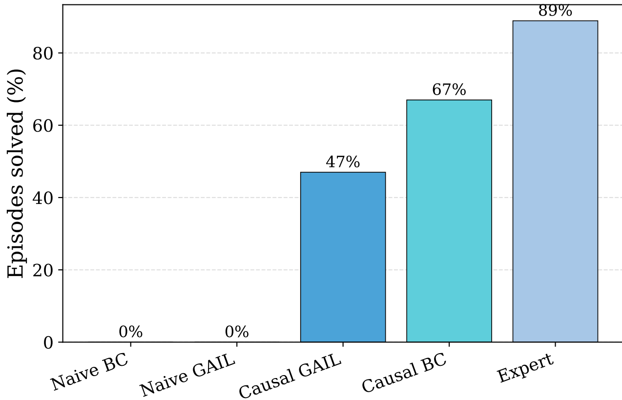
Ant Maze: % episodes solved (< 1000 steps)
