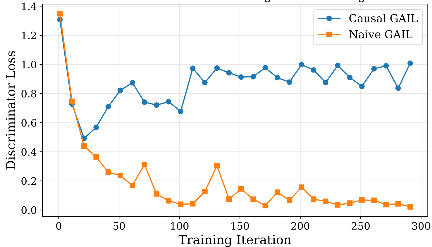
Discriminator Loss During GAIL Training
