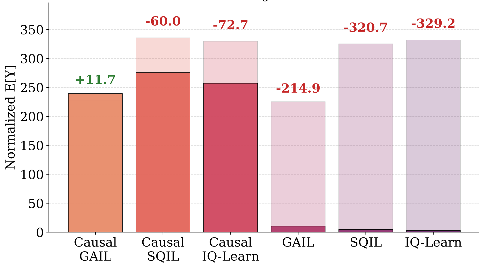
AntMaze Medium: Training vs. Runtime Performance
