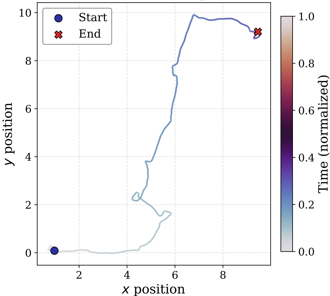
Naive BC (2000 steps)
