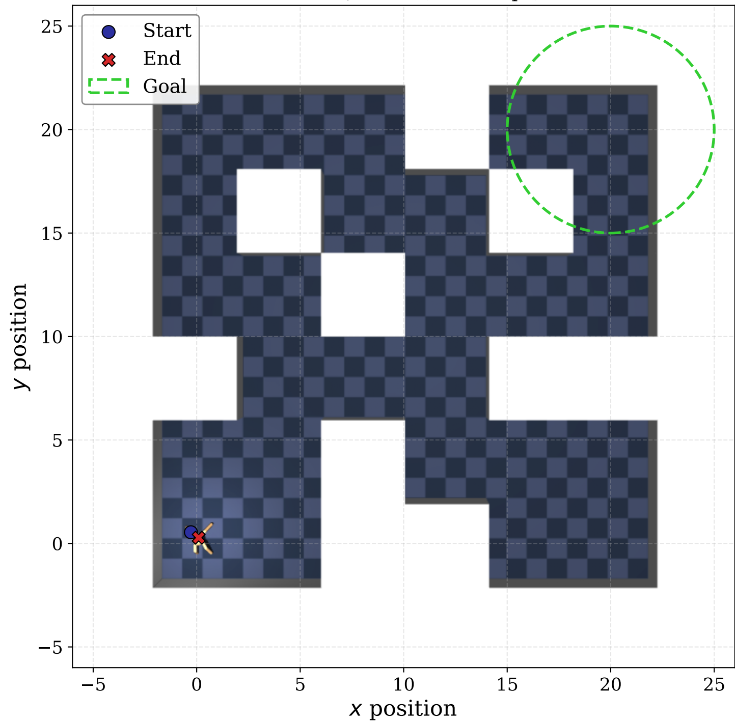
Naive IQ-Learn (1000 steps)
