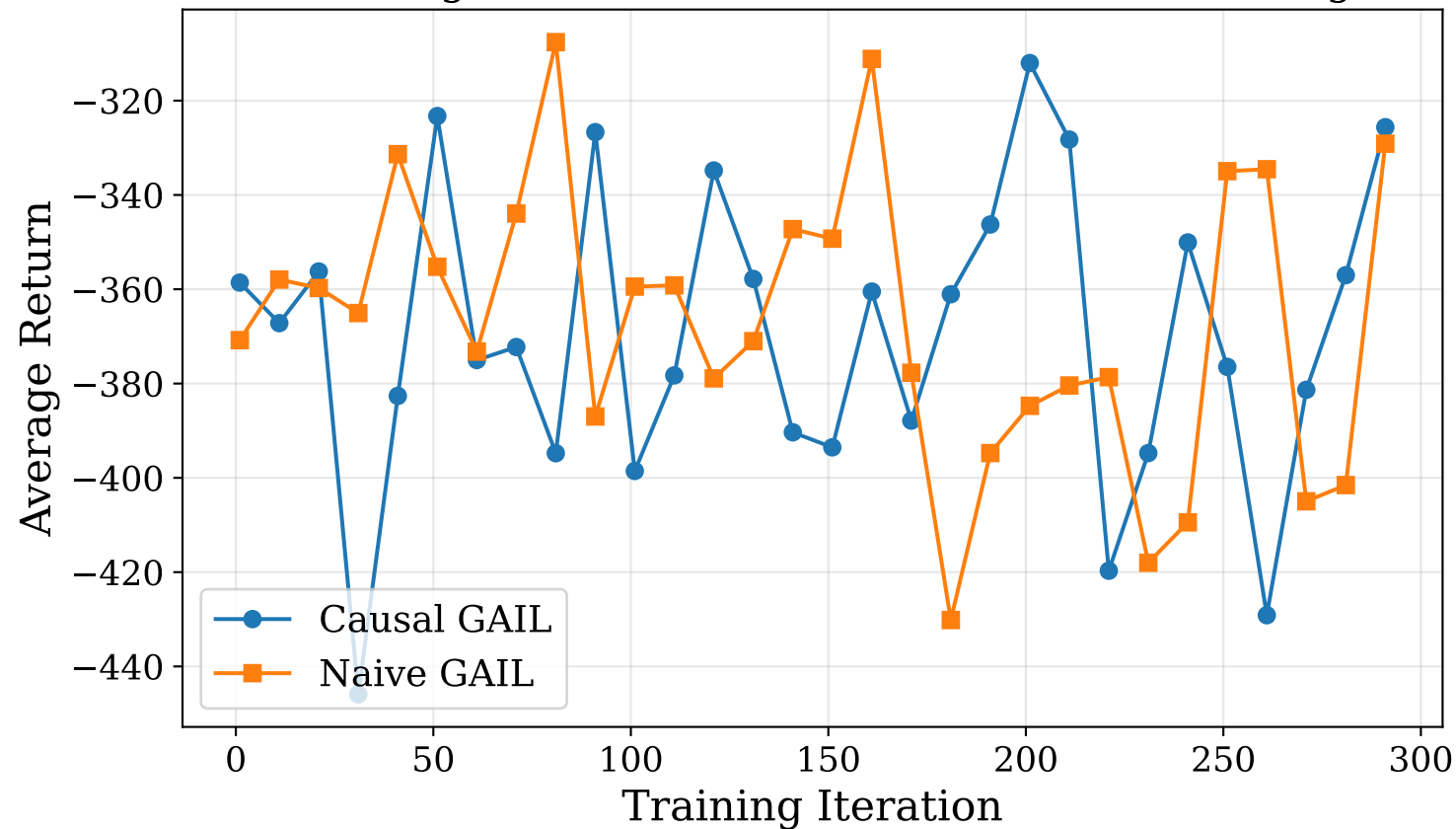
GAIL Training Curve on HumanoidMaze Medium Navigation
