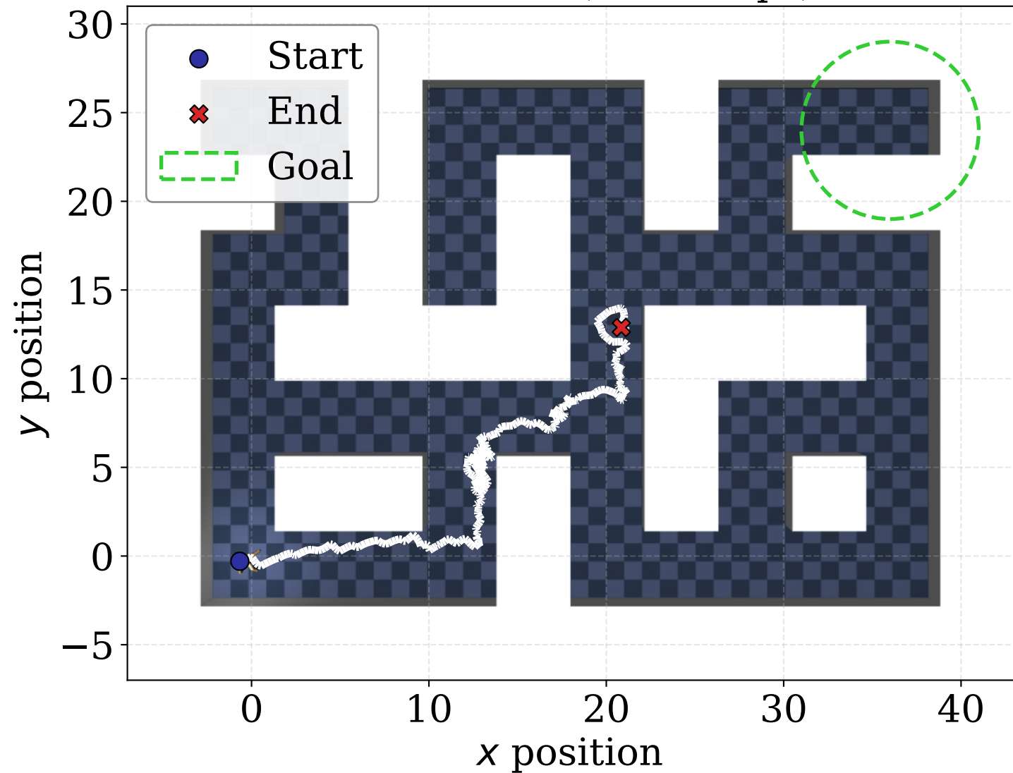
Causal GAIL (1000 steps)
