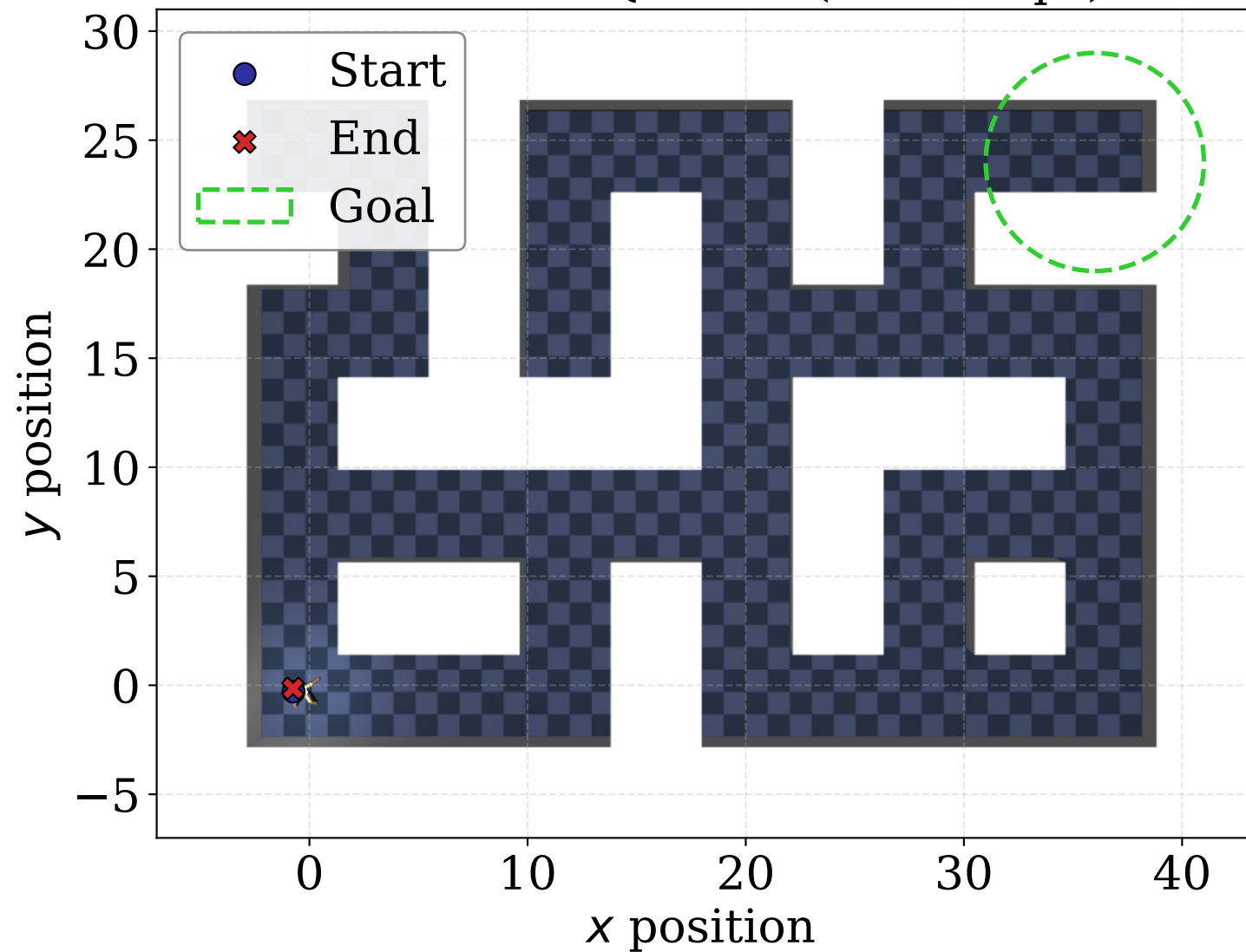
Non-Causal IQ-Learn (1000 steps)
