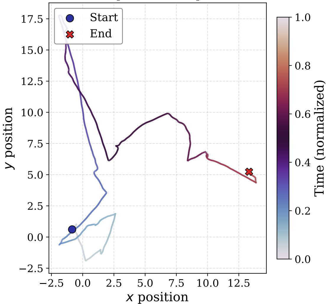
Expert (2000 steps)
