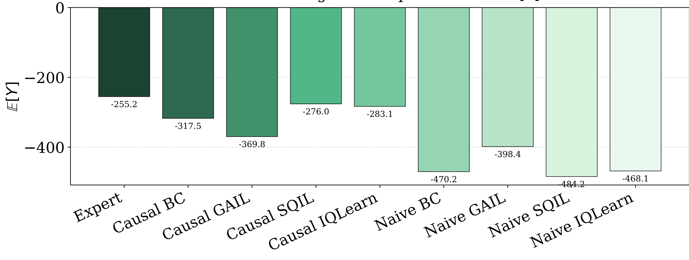
AntMaze Large Mean Episode Return \mathbb{E}[Y]
