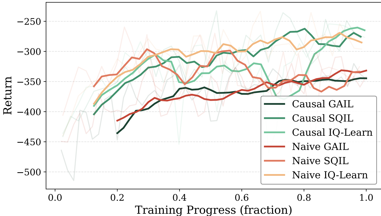
AntMaze Large: All Algorithms
