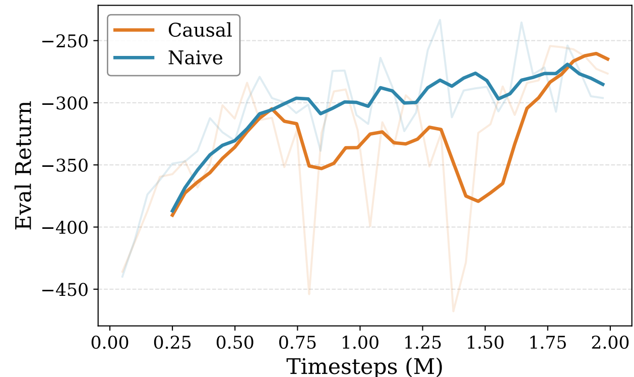
AntMaze Large IQ-Learn
