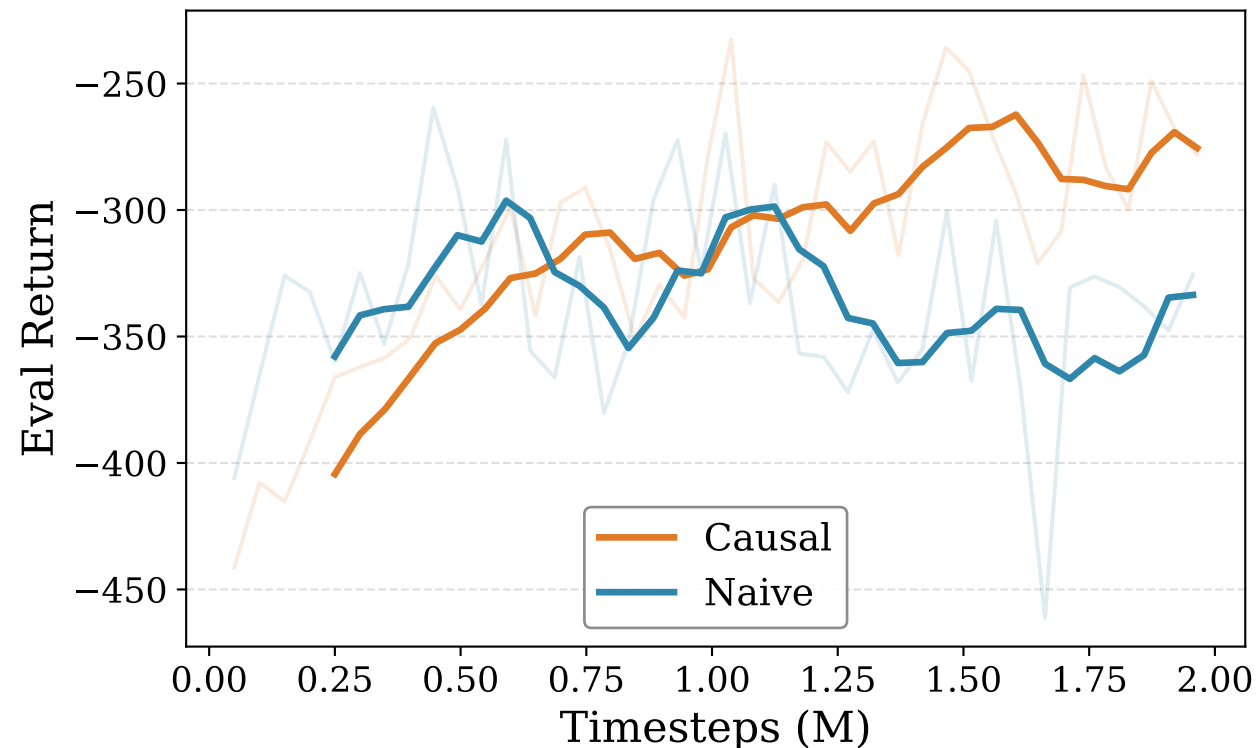
AntMaze Large SQIL
