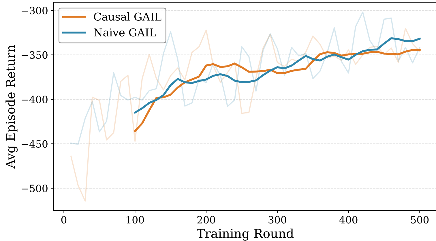
AntMaze Large GAIL: Training Return
