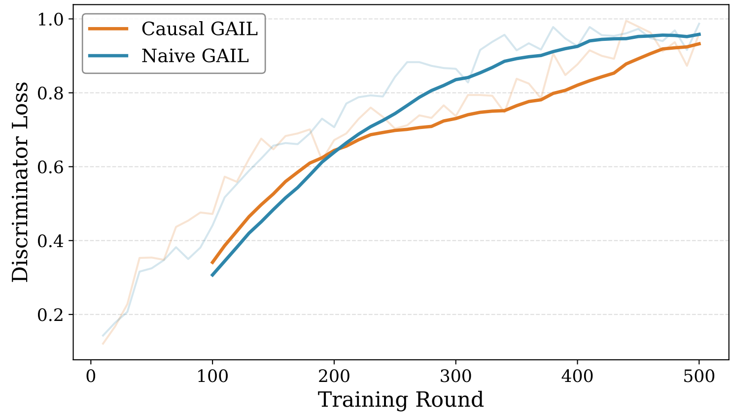
AntMaze Large GAIL: Discriminator Loss
