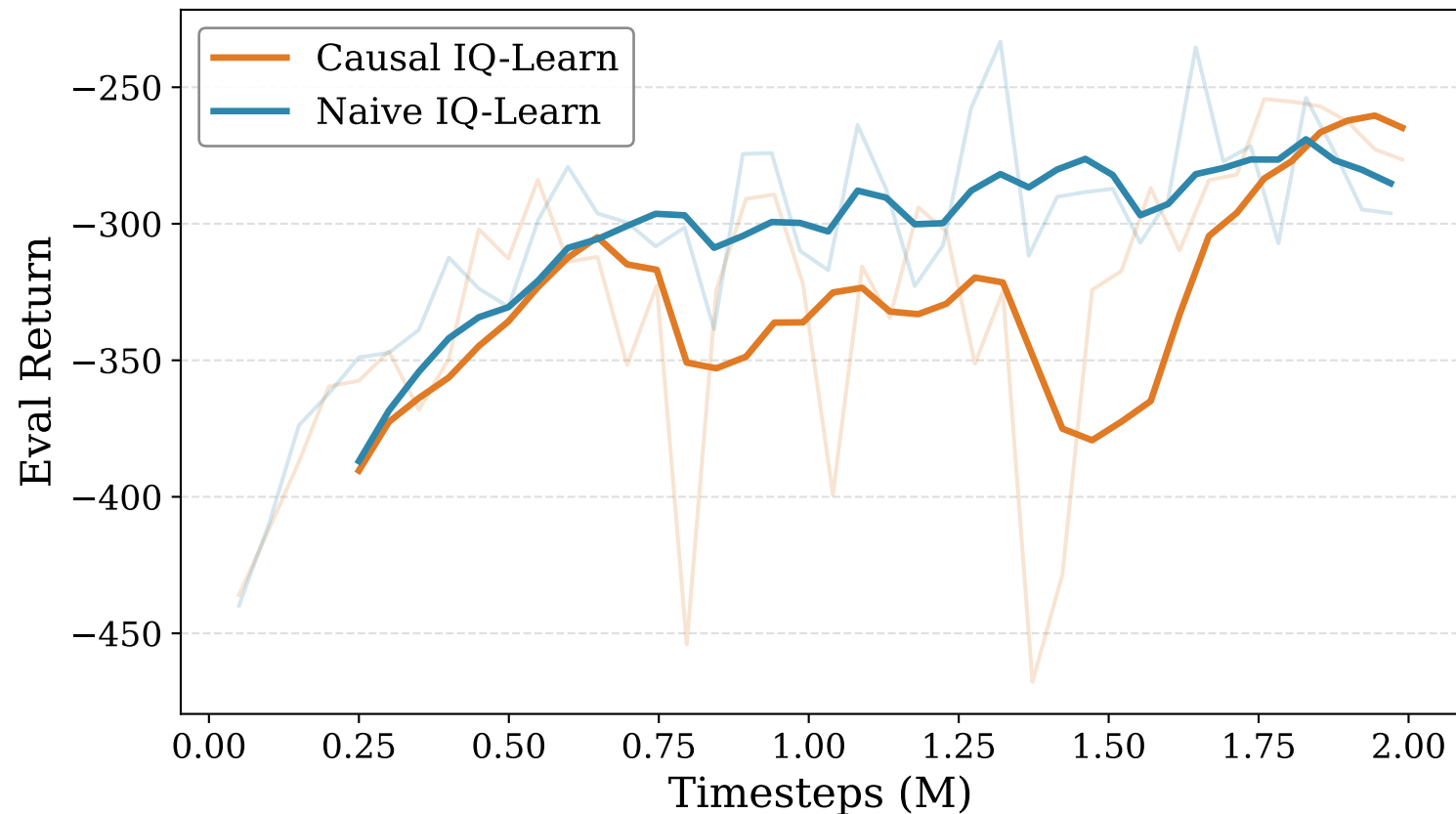
AntMaze Large IQ-Learn: Evaluation Return
