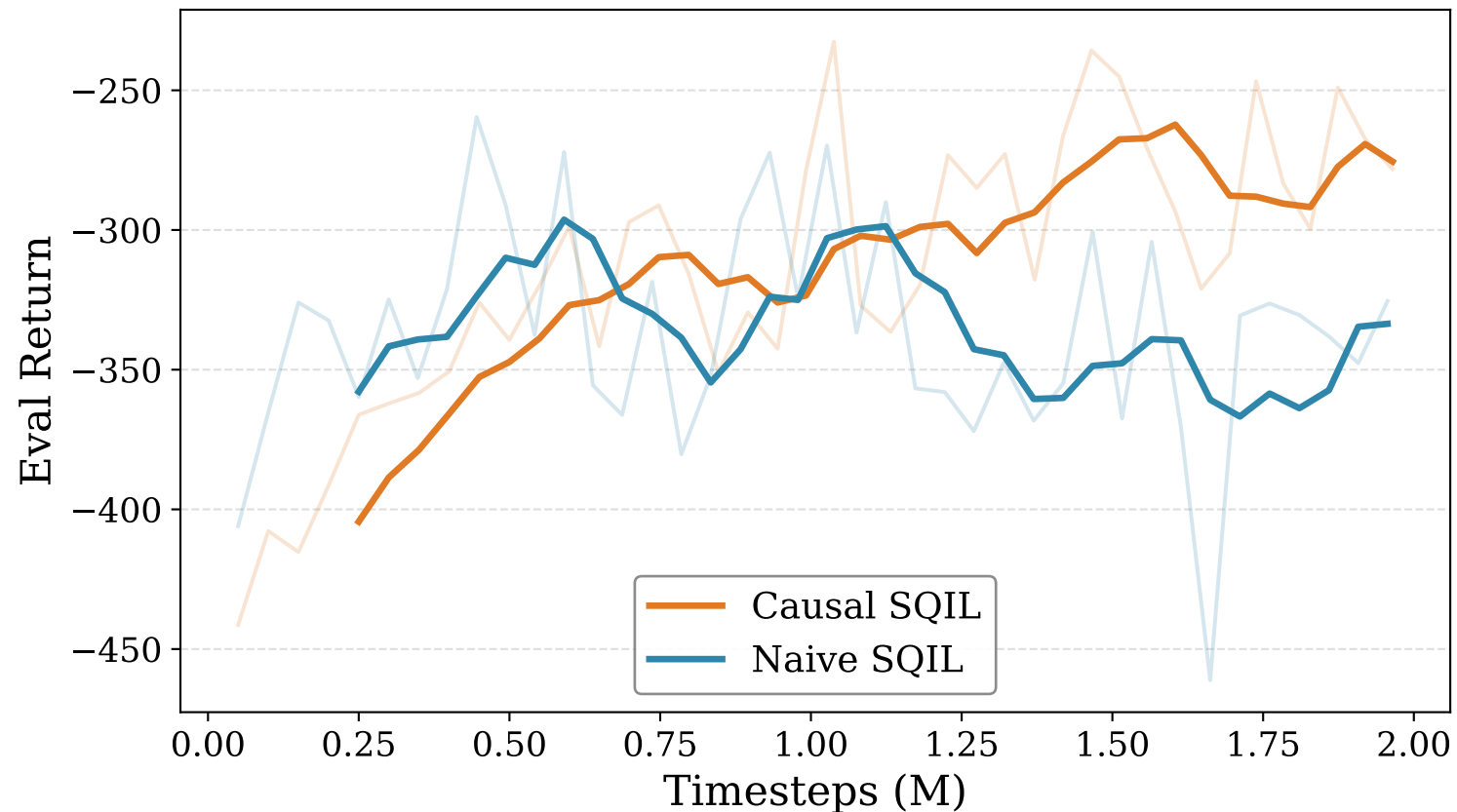
AntMaze Large SQIL: Evaluation Return
