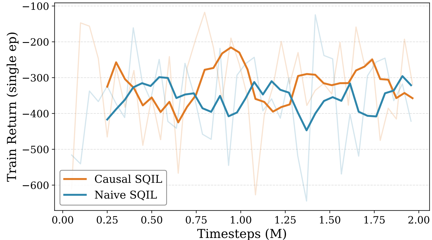
AntMaze Large SQIL: Training Return
