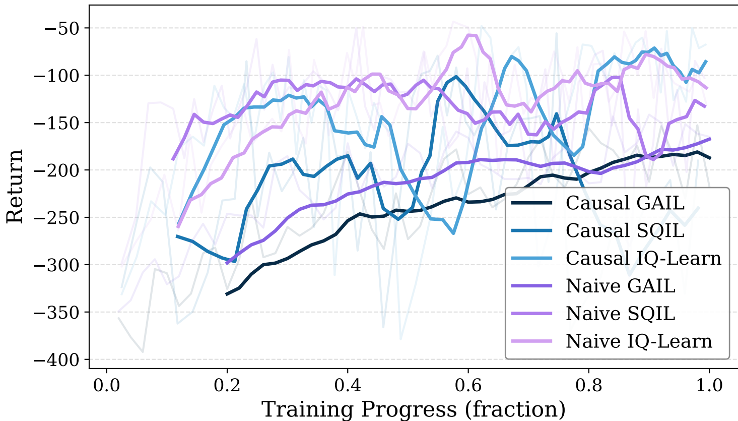
AntMaze Medium: All Algorithms
