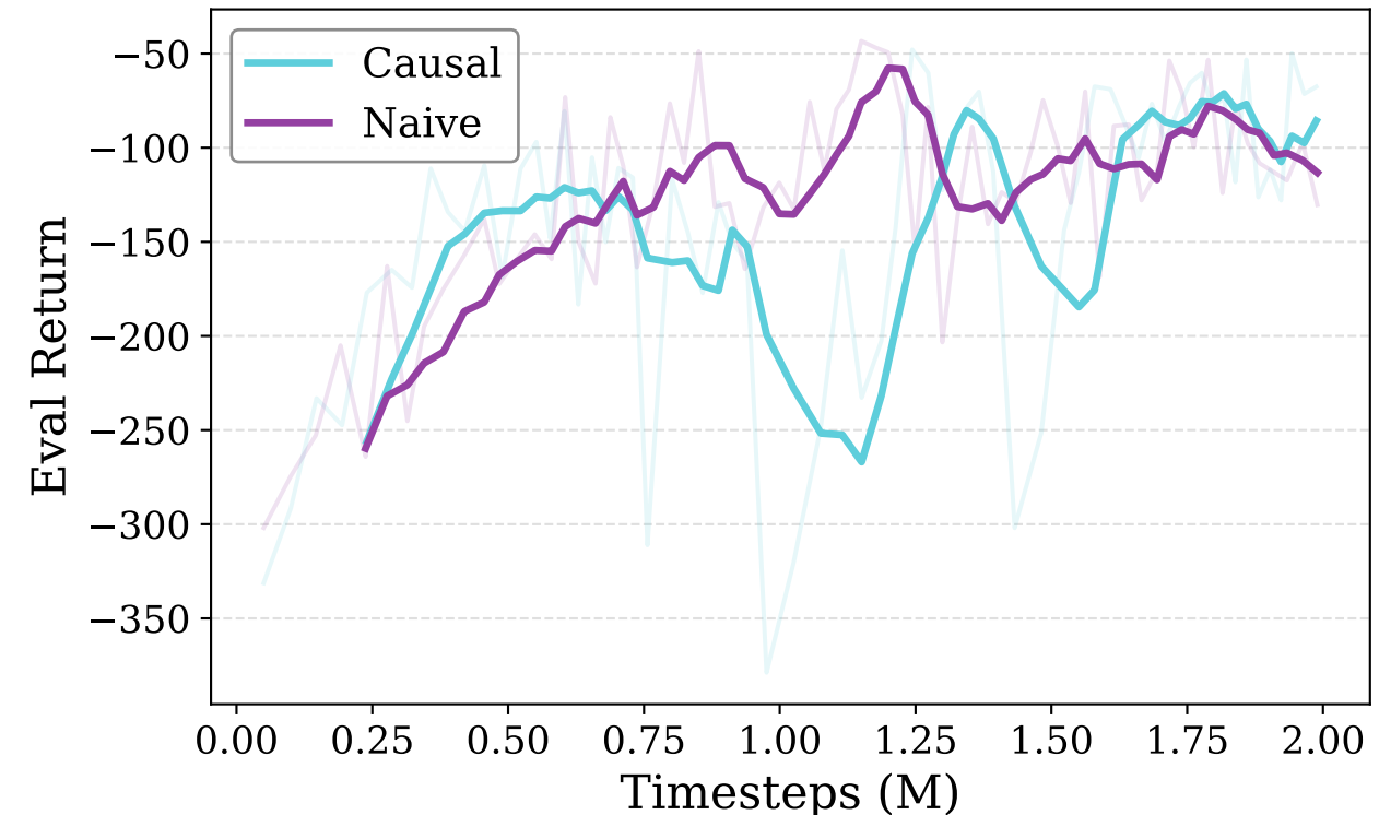
AntMaze Medium IQ-Learn
