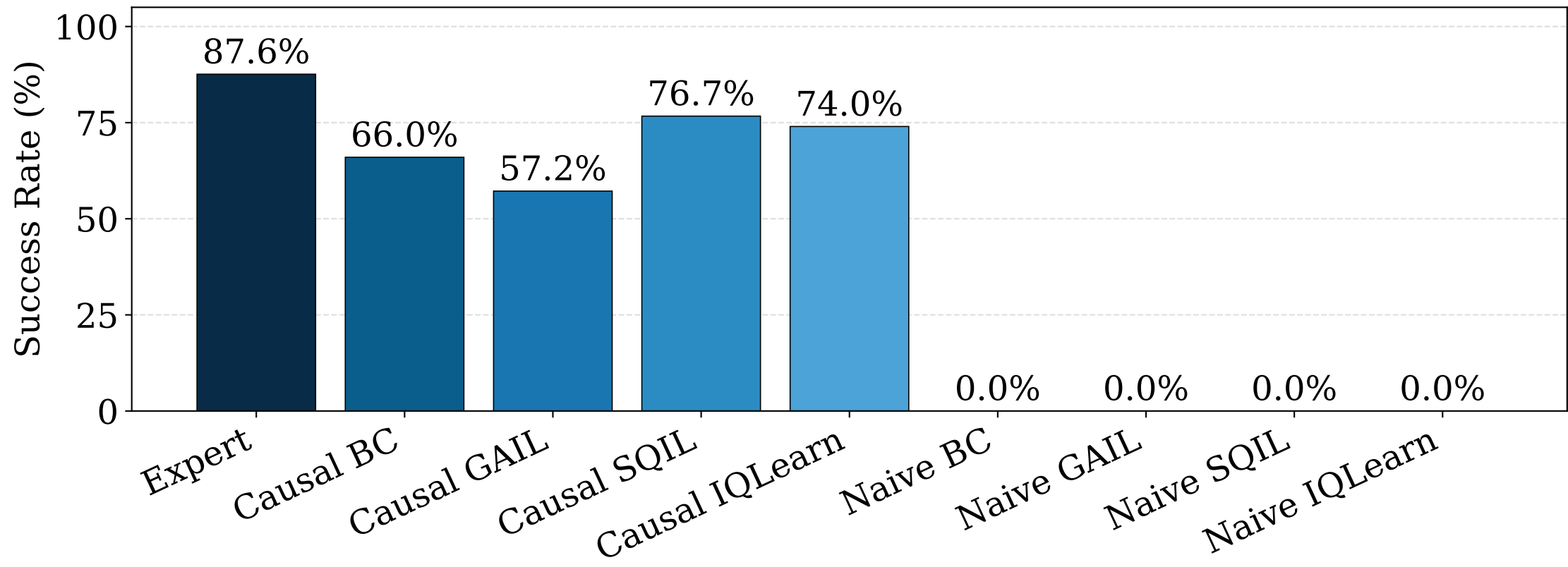
AntMaze Medium Success Rate
