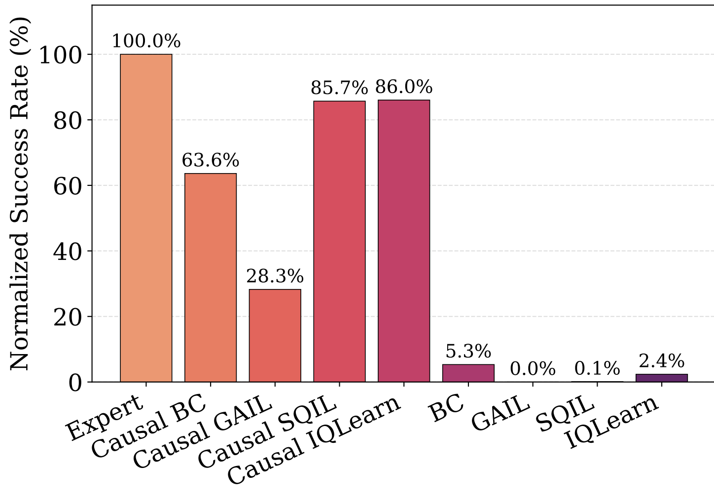
Normalized Success Rate Across Tasks (Expert = 100%)
