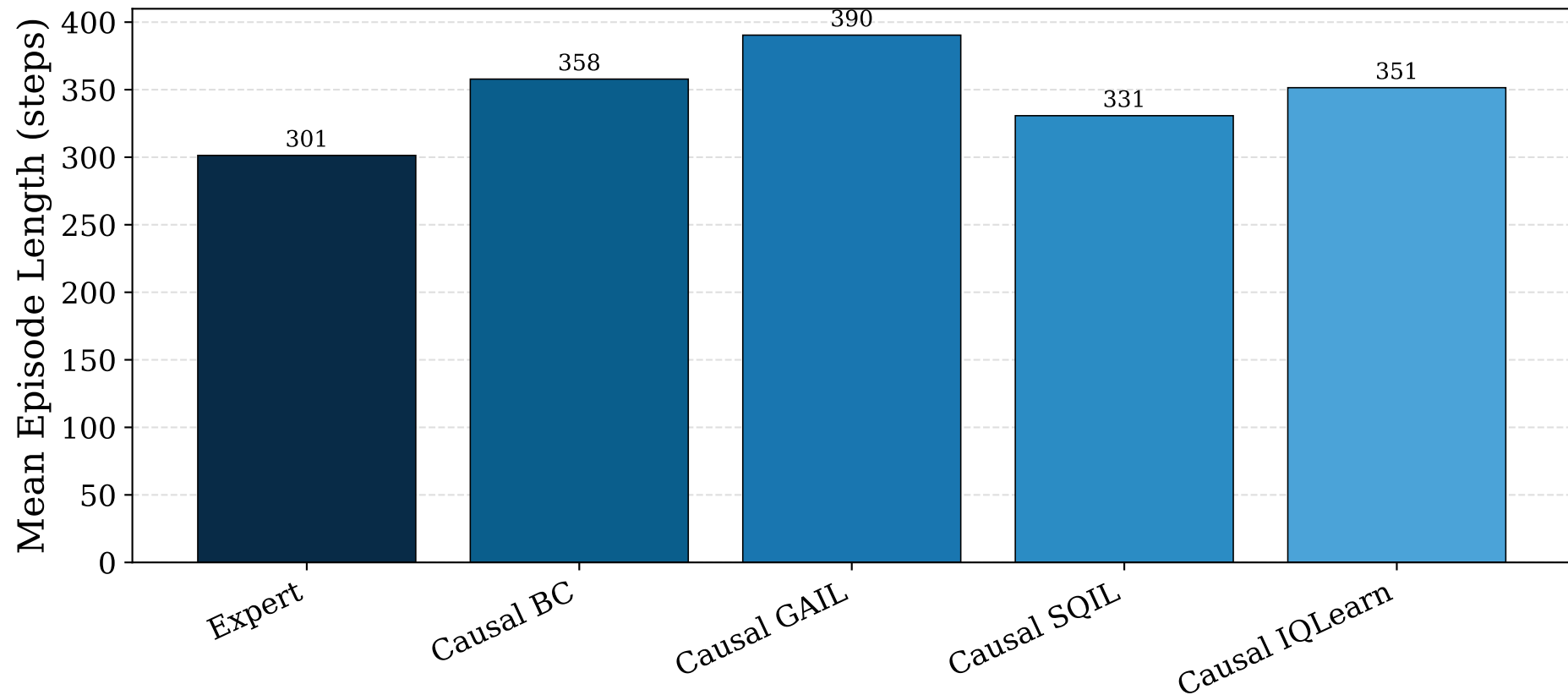
AntMaze Medium Successful Episode Lengths
