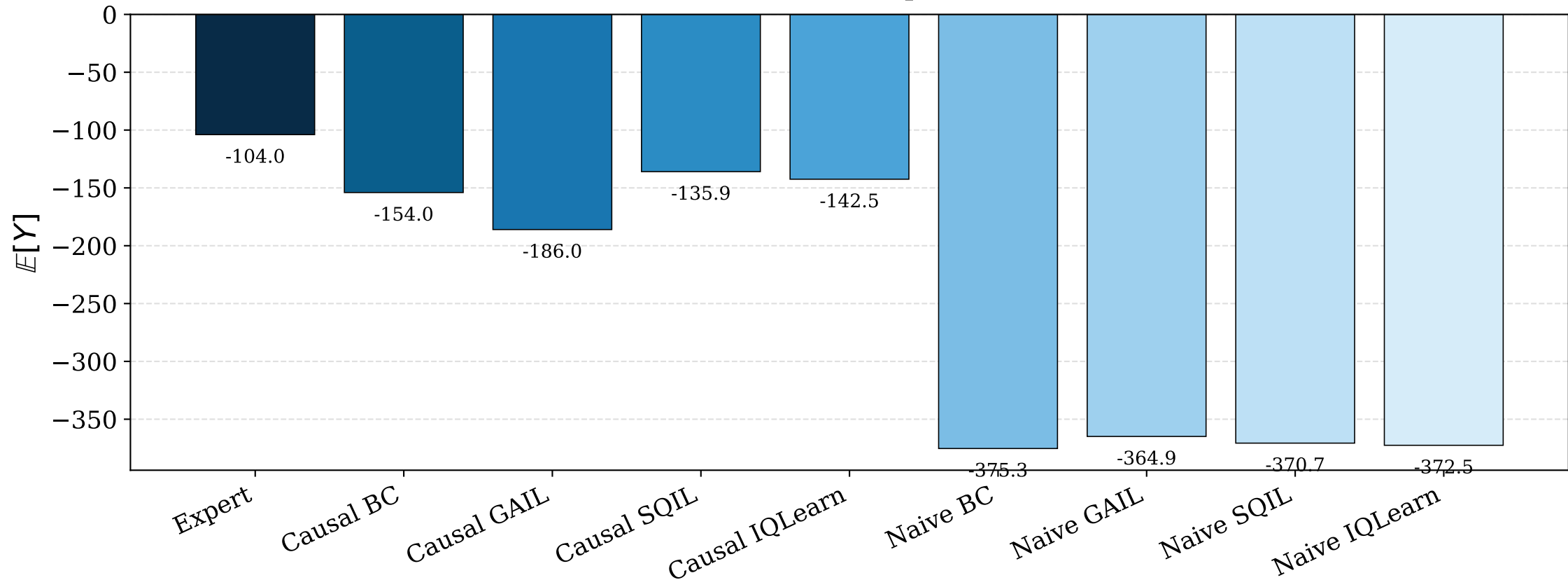
AntMaze Medium Mean Episode Return \mathbb{E}[Y]
