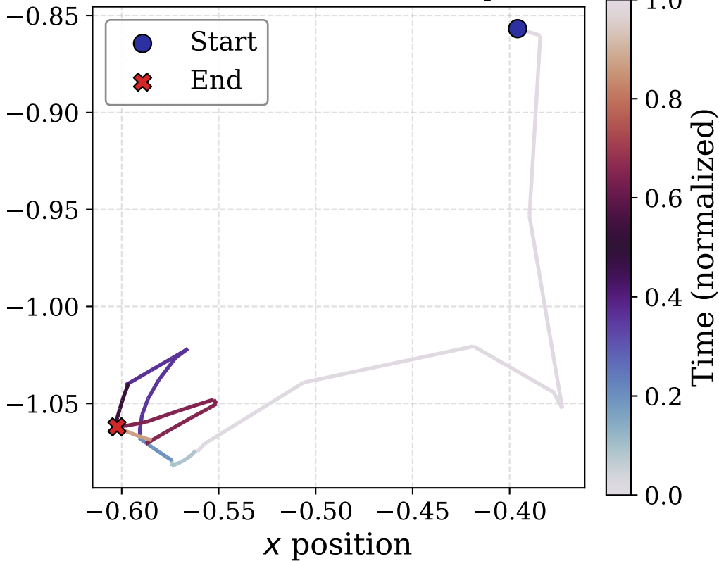
Naive IQLearn (1000 steps)
