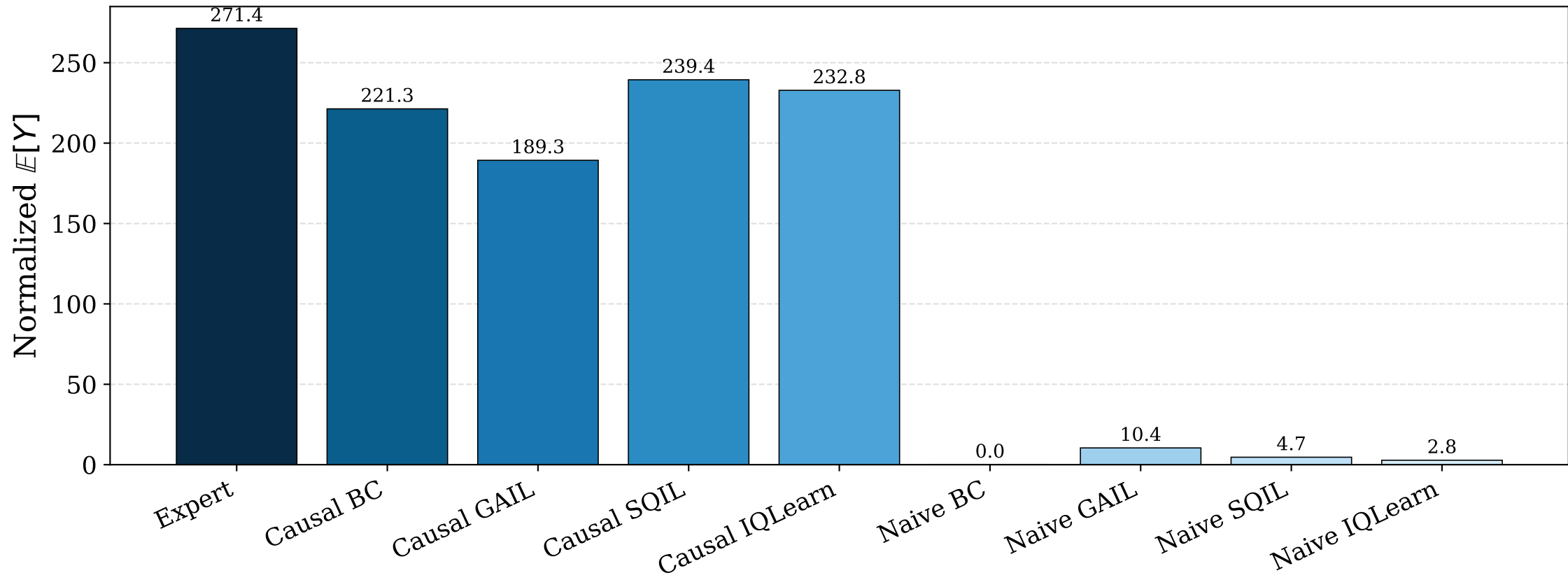
AntMaze Medium Normalized Mean Episode Return
