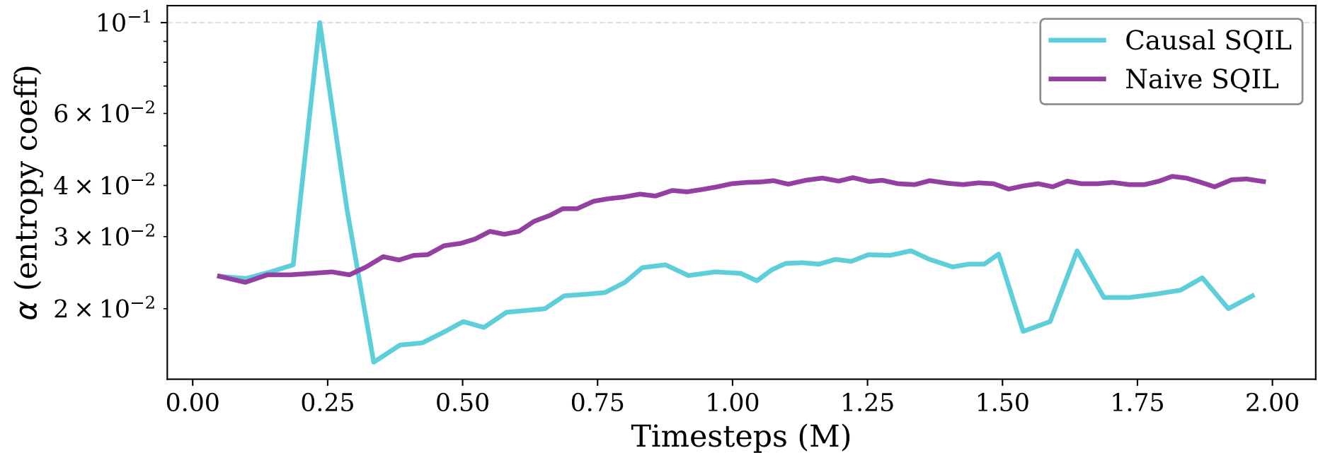
AntMaze Medium SQIL: Entropy Coefficient
