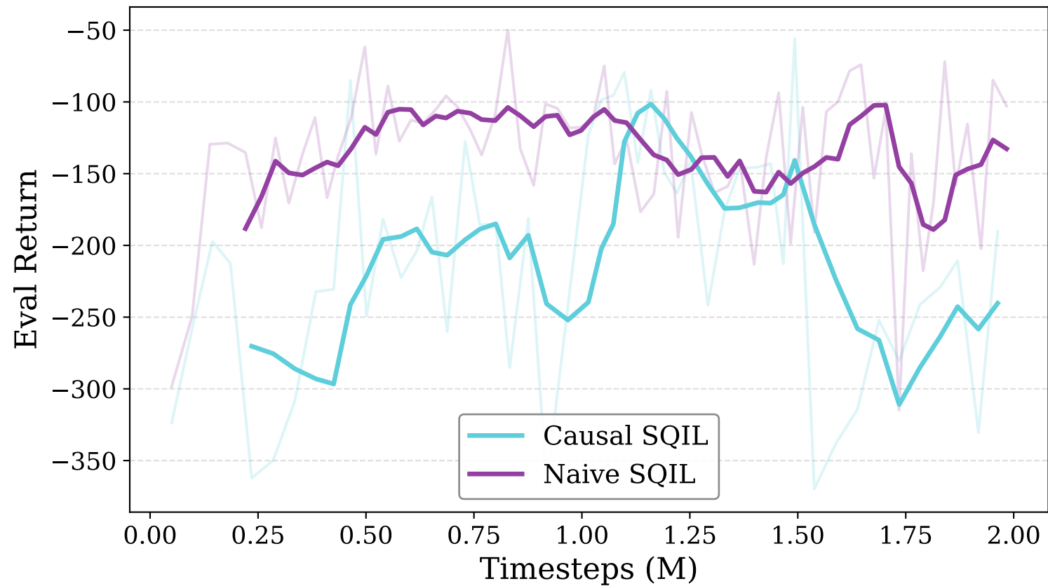
AntMaze Medium SQIL: Evaluation Return
