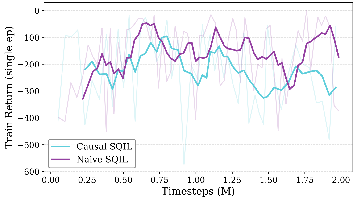
AntMaze Medium SQIL: Training Return
