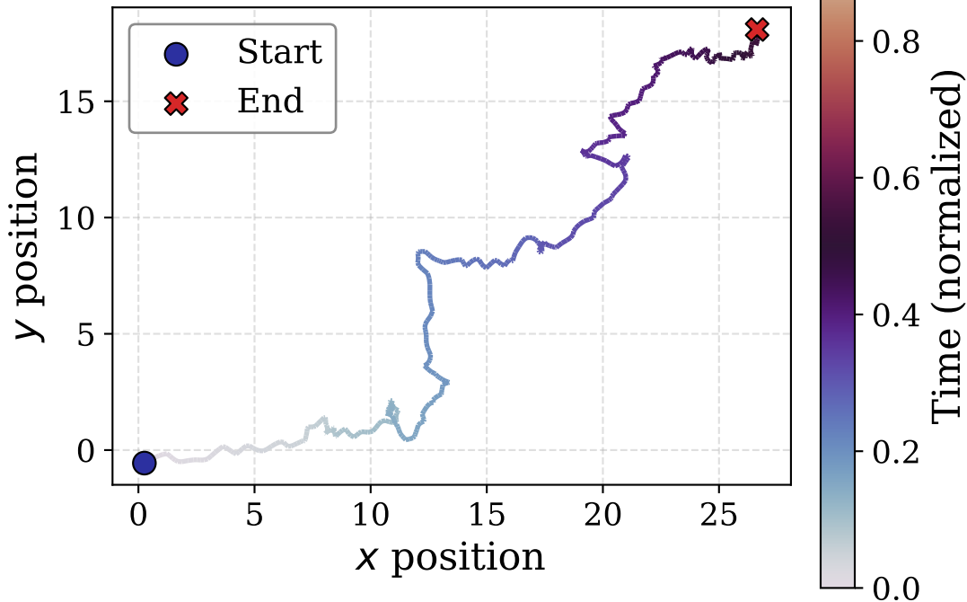
Expert (1000 steps)
