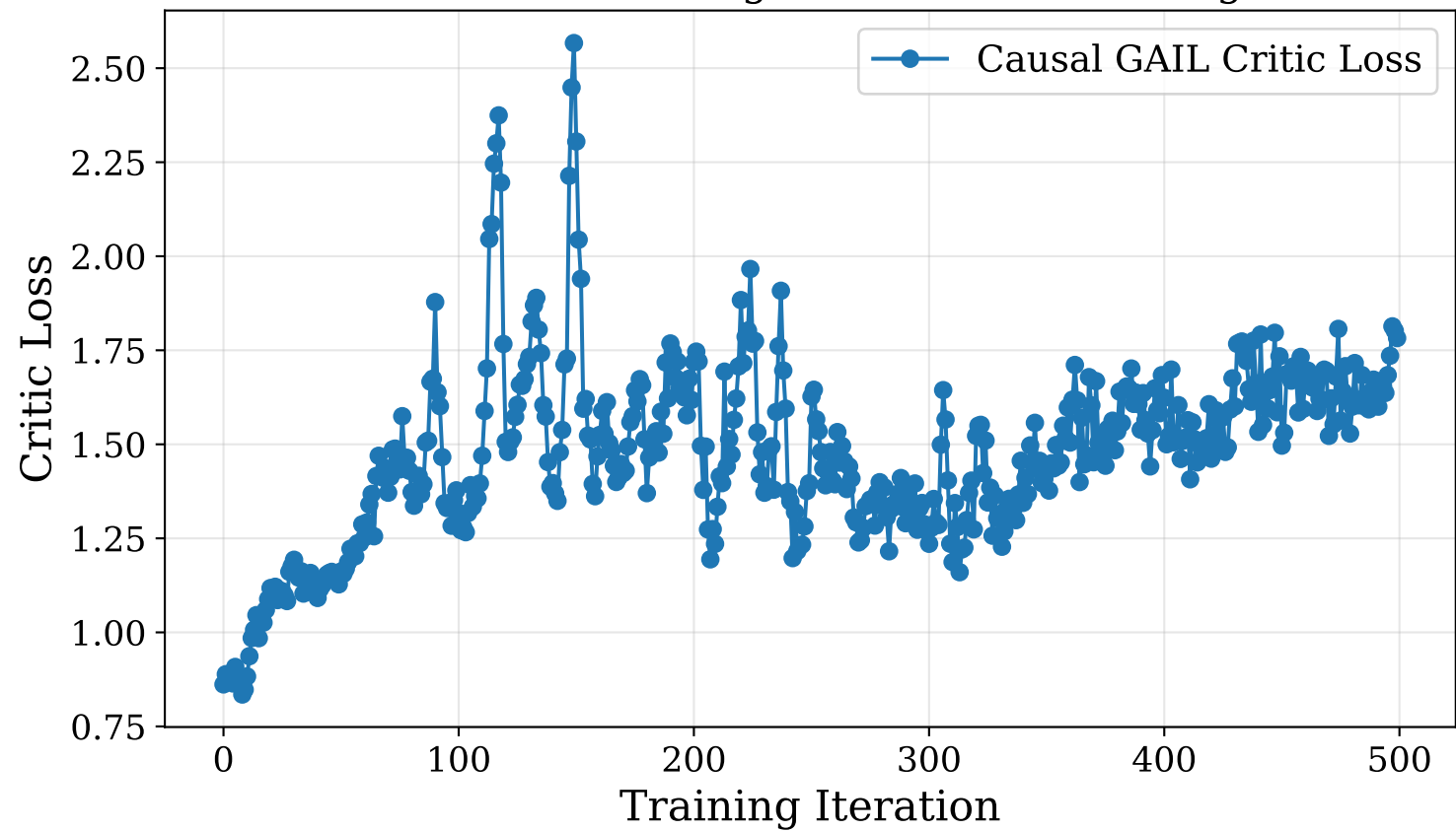
Critic Loss During Causal GAIL Training
