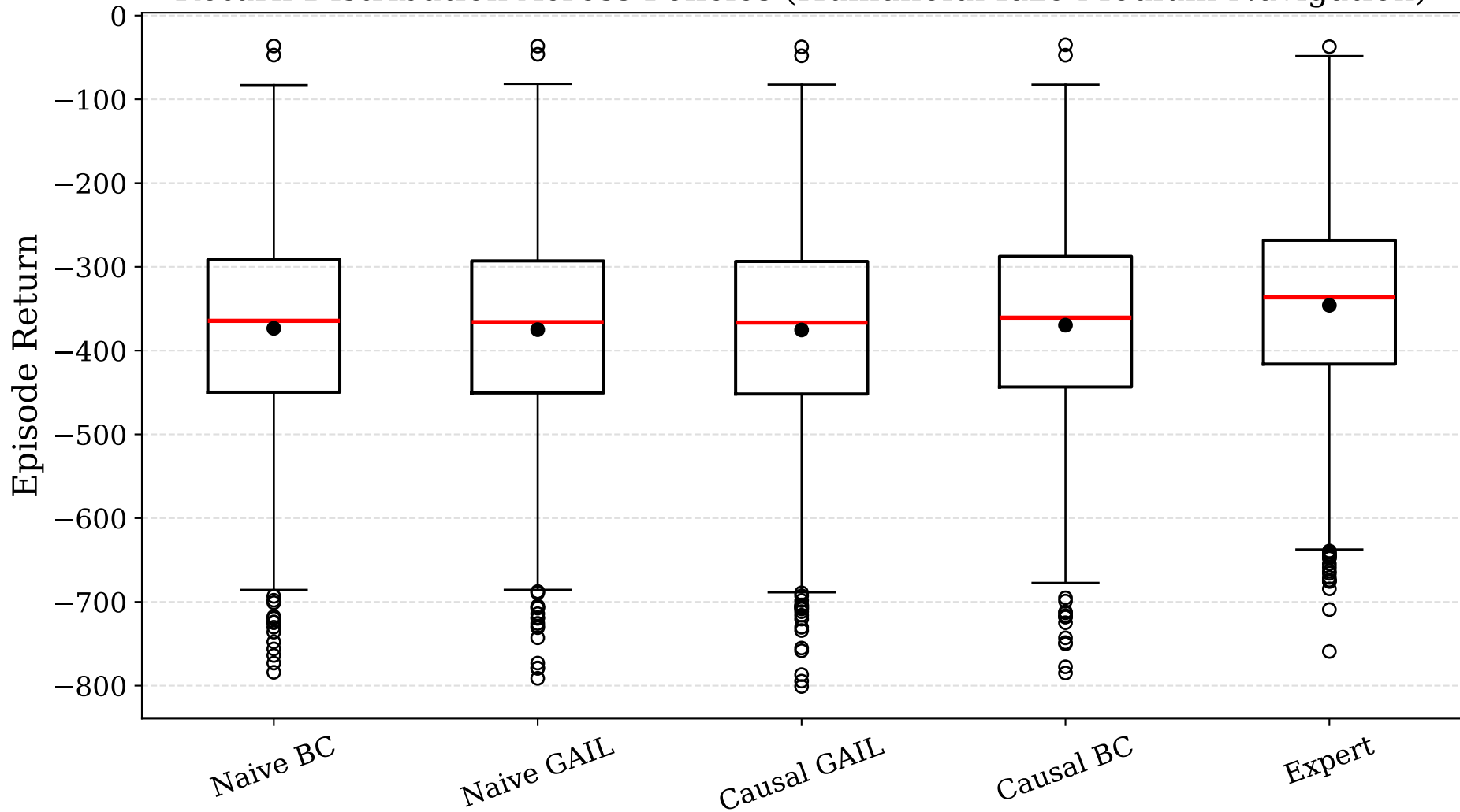
Return Distribution Across Policies (HumanoidMaze Medium Navigation)
