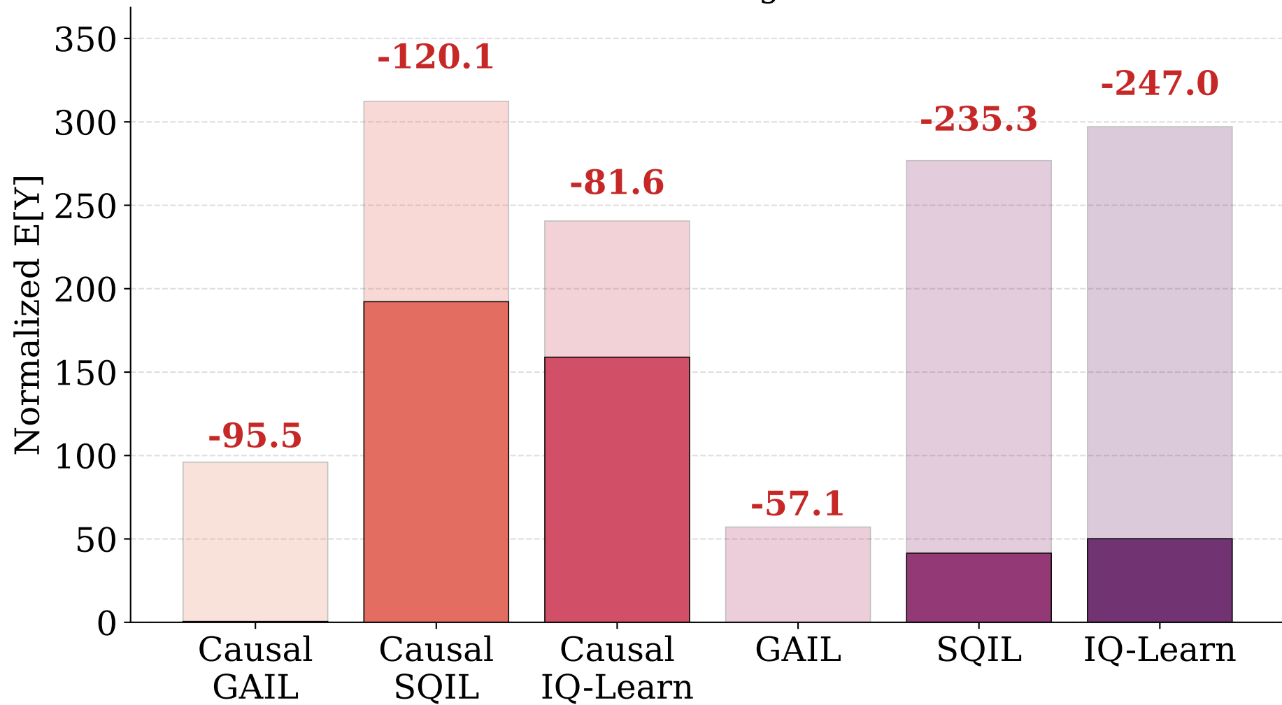
HumanoidMaze Medium: Training vs. Runtime Performance
