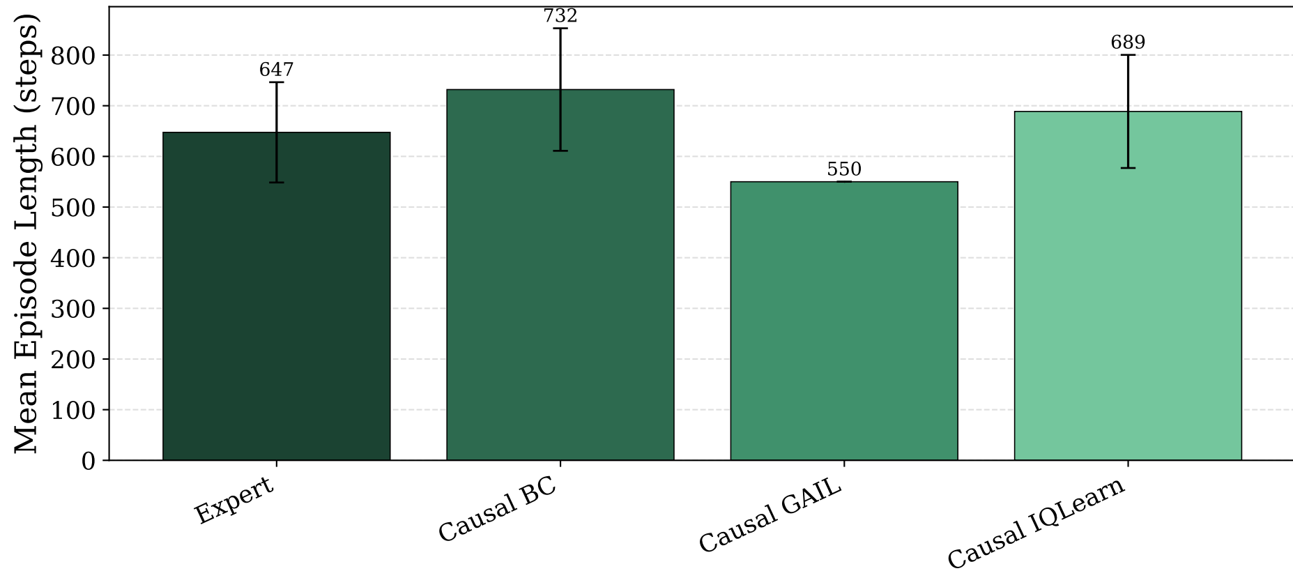
AntMaze Large Successful Episode Lengths ( \pm Std)
