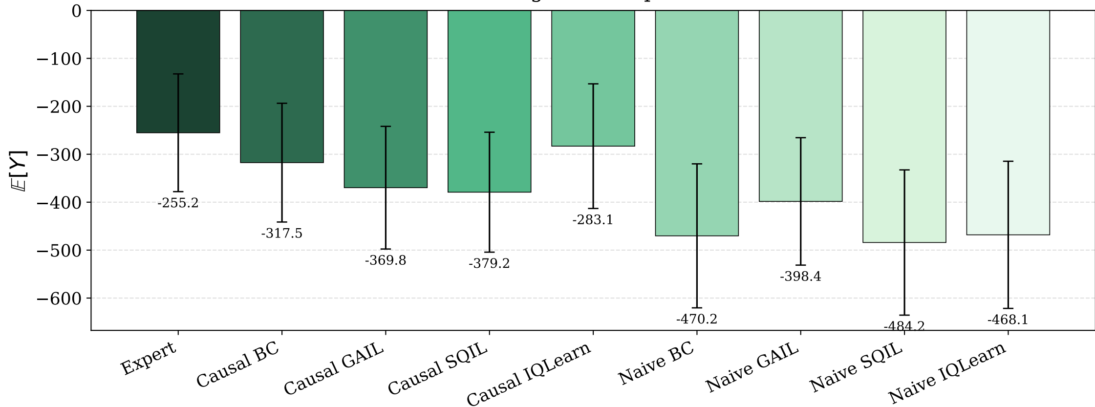
AntMaze Large Mean Episode Return
