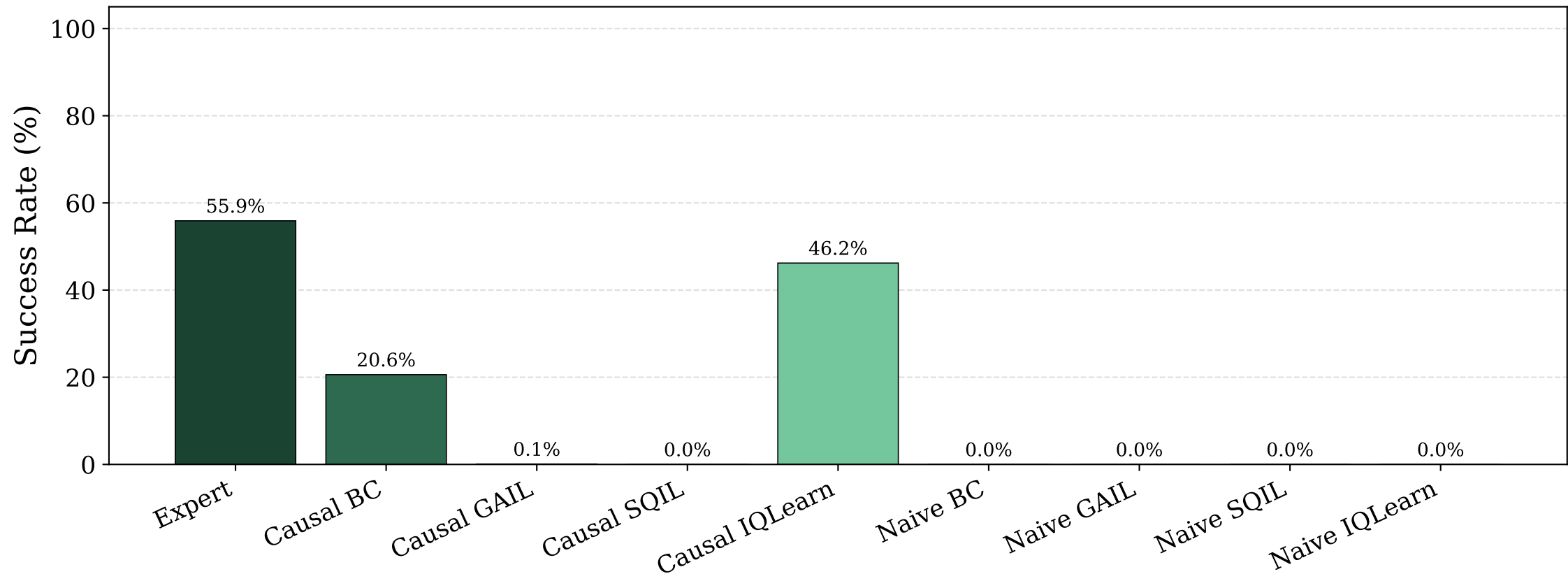
AntMaze Large Success Rate
