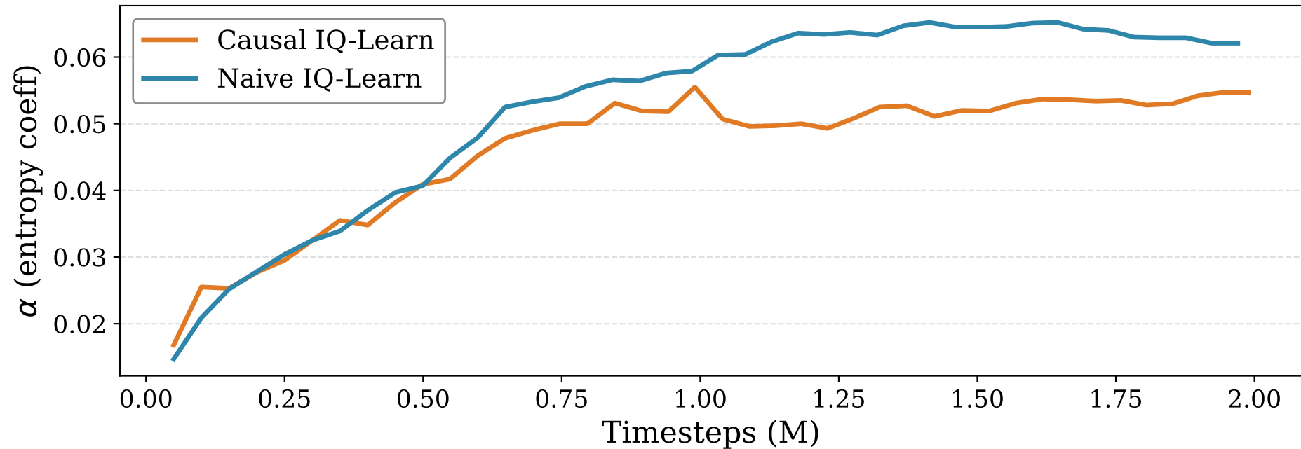
AntMaze Large IQ-Learn: Entropy Coefficient
