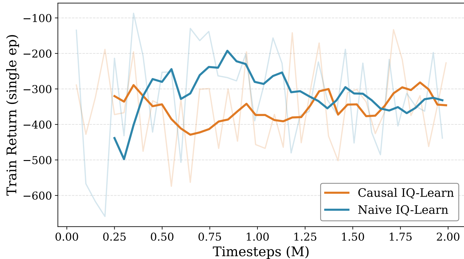
AntMaze Large IQ-Learn: Training Return
