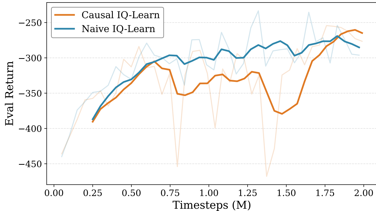
AntMaze Large IQ-Learn: Evaluation Return
