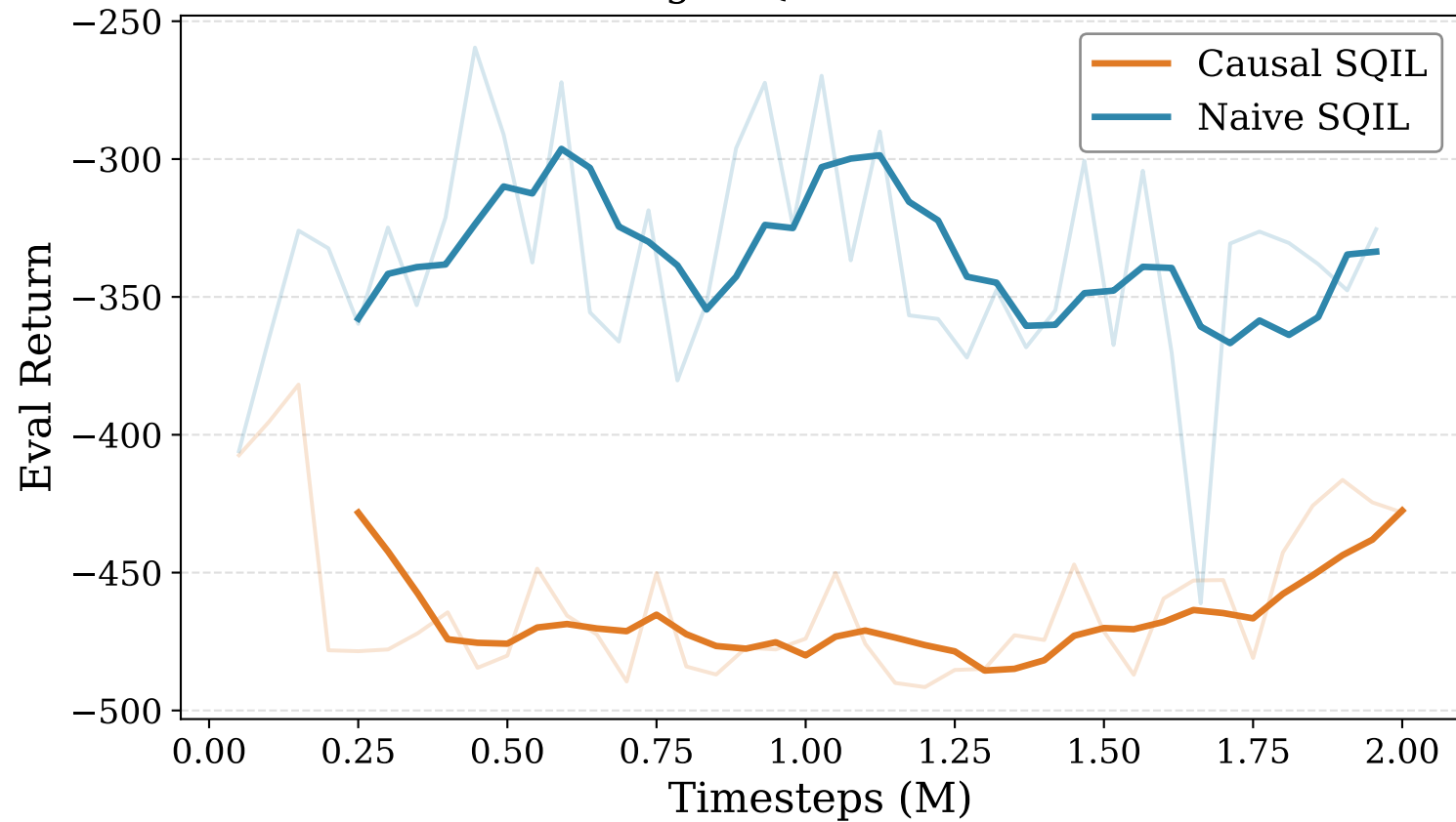
AntMaze Large SQIL: Evaluation Return
