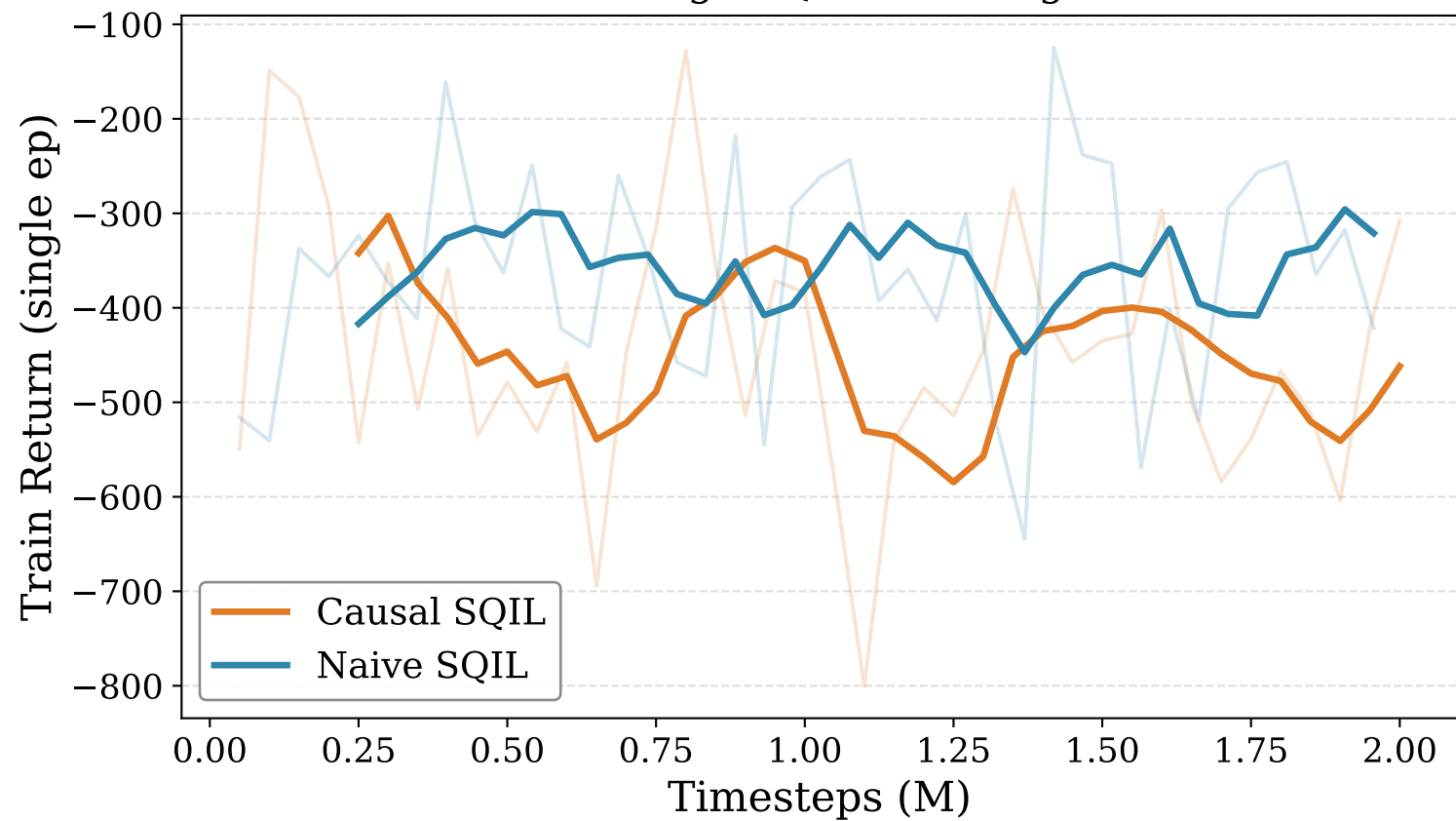
AntMaze Large SQIL: Training Return
