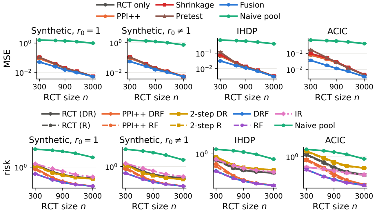
Figure 7: Absolute errors for the designs of Fig. 4, columns 1–4. Top: ATE MSE; bottom: CATE risk. 95% bootstrap intervals.
