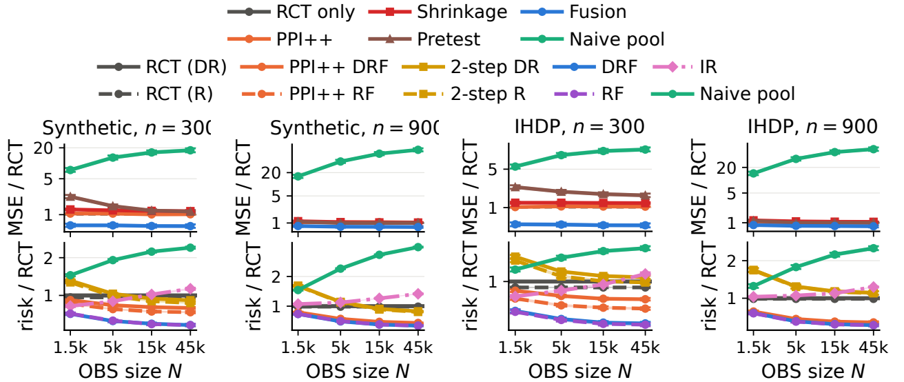
Figure 6: Effect of the observational sample size N (split 60/20/20) under the covariate shift, for the synthetic design and IHDP at n = 300 and 900 . Top: ATE MSE relative to RCT only; bottom: CATE risk relative to the trial-only DR-learner. 95% bootstrap intervals.
