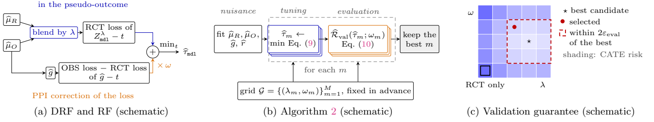
Figure 3: CATE fusion with DRF and RF. (a) Where \lambda and \omega enter the loss (Def. 3). (b) Algorithm 2. (c) Thm. 4: shading is the CATE risk; the selected candidate is within 2\varepsilon_{\text{eval}}(\alpha) of the best (dashed) when \hat{r} = r_0 .
