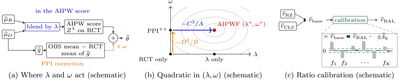
Figure 2: ATE fusion with AIPWF (Def. 1). (a) Where \lambda and \omega enter \hat{\theta} . (b) Contours of Eq. (4). (c) Ratio calibration (Def. 2): bars are the imbalances \mathbb{P}_O^{\text{nuis}}[\hat{r}f_k] - \mathbb{P}_R^{\text{nuis}}[f_k] .
