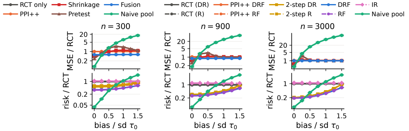
Figure 5: Bias sweep on the synthetic design under the strong shift at n = 300, 900 , and 3,000 , against the confounding bias in units of \text{sd}_R \tau_0(X) . Top: ATE MSE relative to trial-only AIPW; bottom: CATE risk relative to the trial-only DR-learner. 95% bootstrap intervals.
