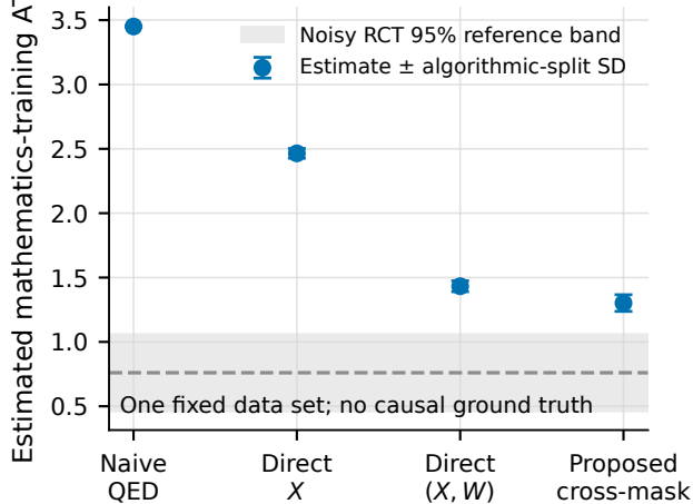
WSC observational benchmark
