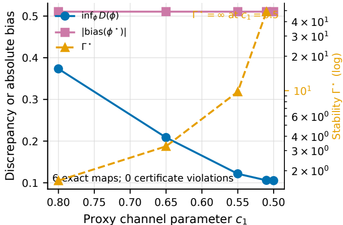
Finite-state certificate
