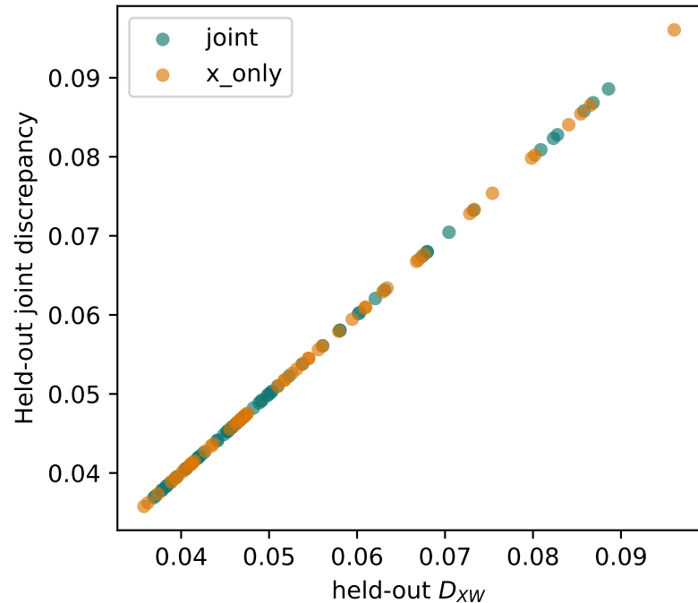
Held-out joint discrepancy
