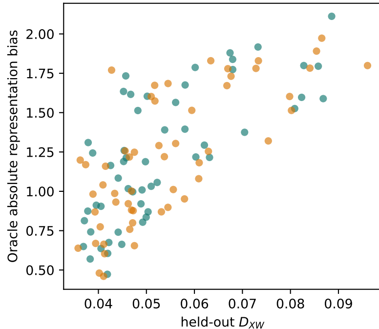
Oracle absolute representation bias
