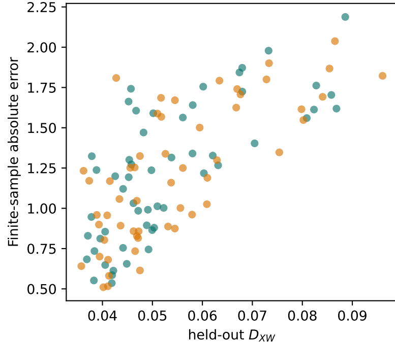
Finite-sample absolute error
