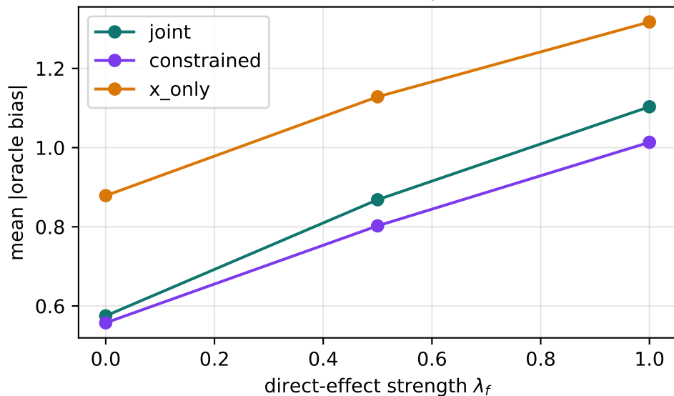
Tabular direct-X (36 pairs/level)
