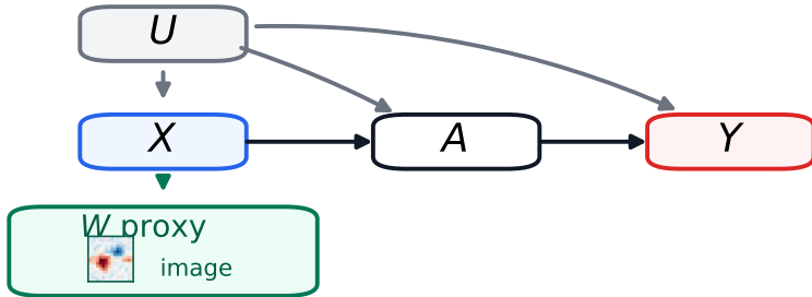
Image 1. data-generating graph
