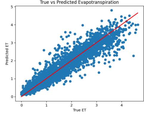
Fig. 14. LSTM Regression Predictions vs. Ground Truth
