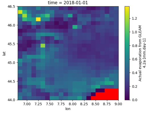
Fig. 10. Spatial Points of the Filtered GLEAM Dataset
