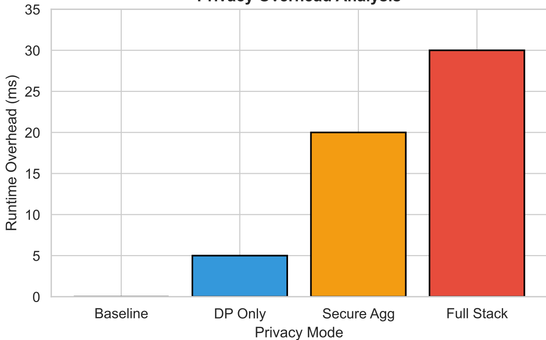
Privacy Overhead Analysis
