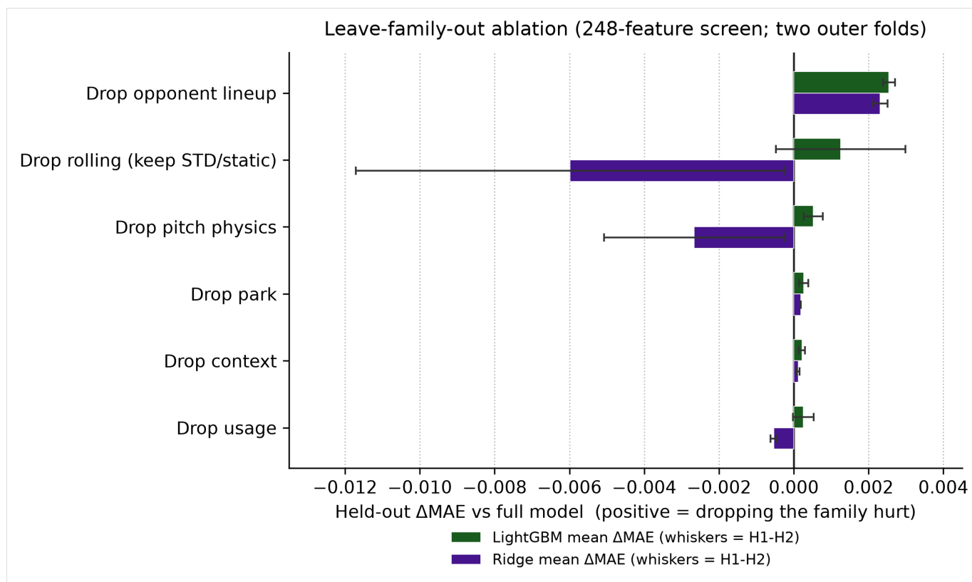
Figure 3. Leave-family-out mean \Delta MAE for LightGBM and Ridge with whiskers spanning the two outer folds (H1-H2). Positive values indicate that removing the family increased held-out error. Wide whiskers (especially Ridge rolling / physics) show that the two-fold mean alone can mislead. Table 6 remains authoritative.
