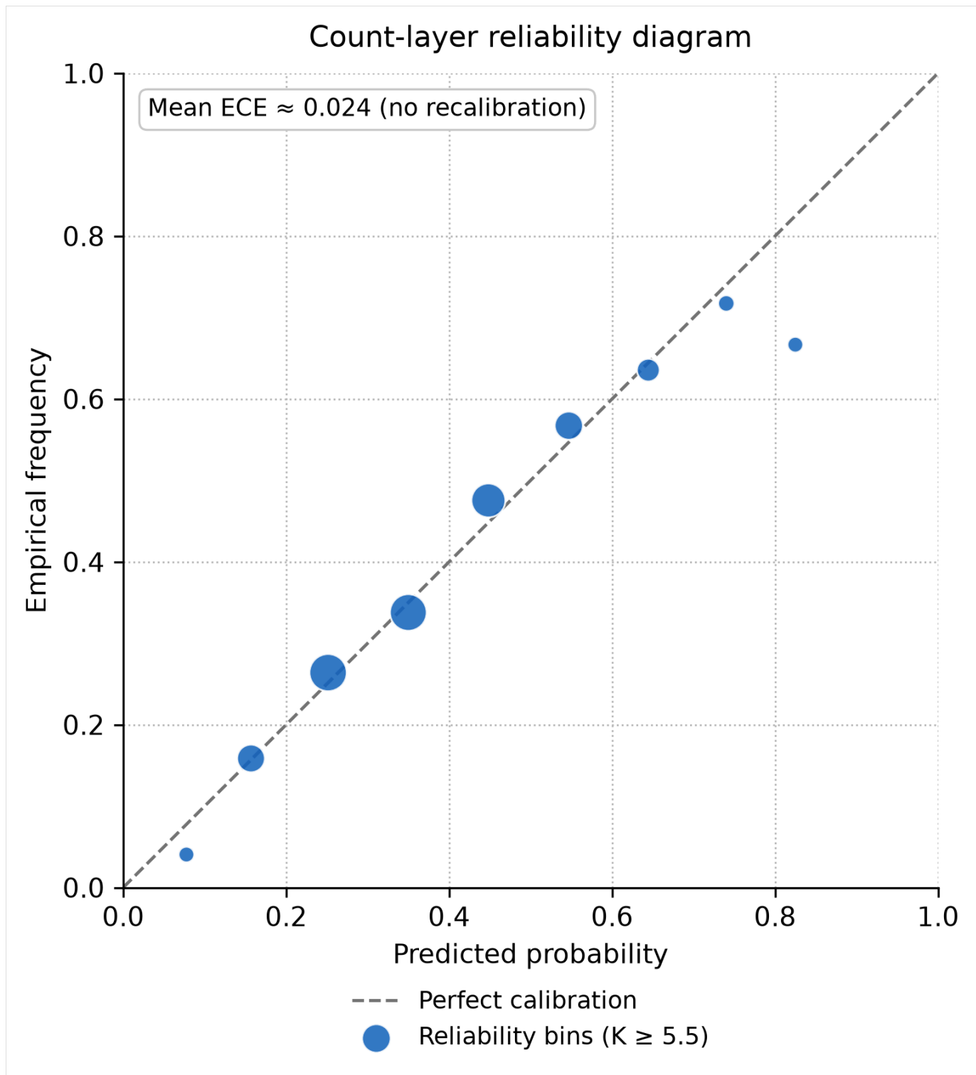
Figure 4. Reliability diagram for count-layer line probabilities. Points near the diagonal indicate well-calibrated bins; the manuscript reports mean ECE \approx 0.024 with no post-hoc recalibration. Calibration is internal to the chronological test; it is not a market benchmark.
