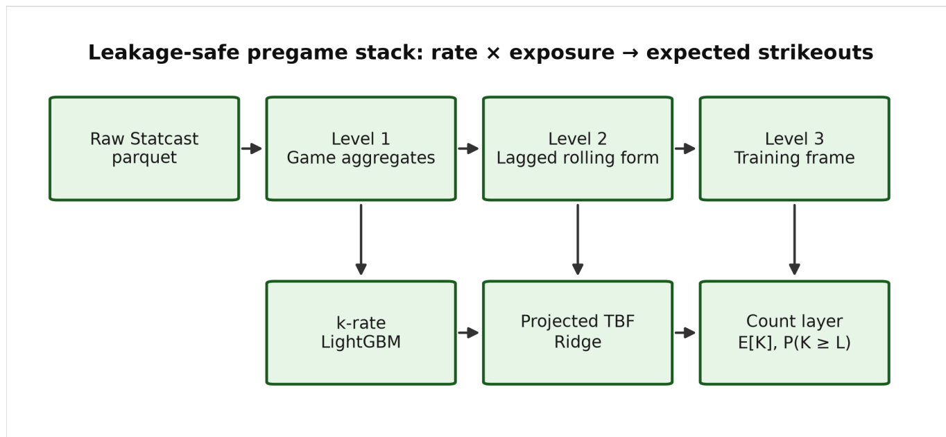
Figure 1. Leakage-safe architecture. Raw Statcast pitches are aggregated into game records (Level 1), lagged rolling form (Level 2), and a model-ready training frame (Level 3). A LightGBM strikeout-rate model and a Ridge projected-TBF model combine in a count layer that yields expected strikeouts and line probabilities from projected exposure only.
