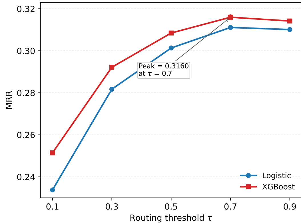
(a) MRR versus routing threshold
