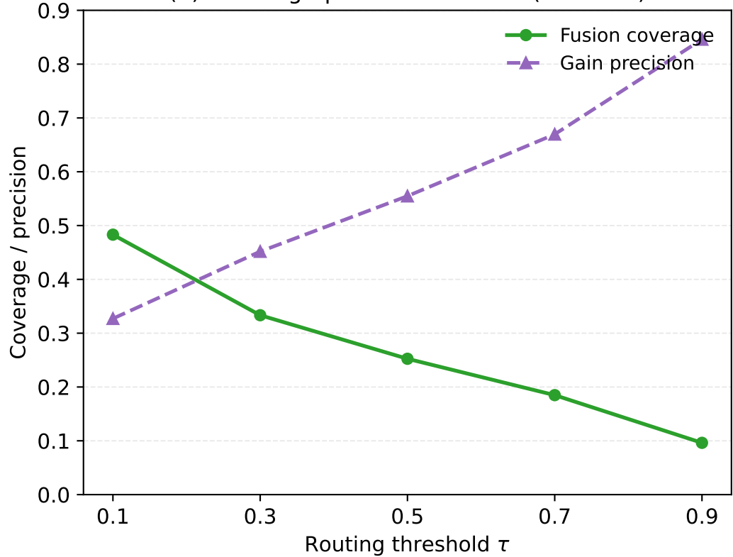
(b) Coverage-precision tradeoff (XGBoost)
