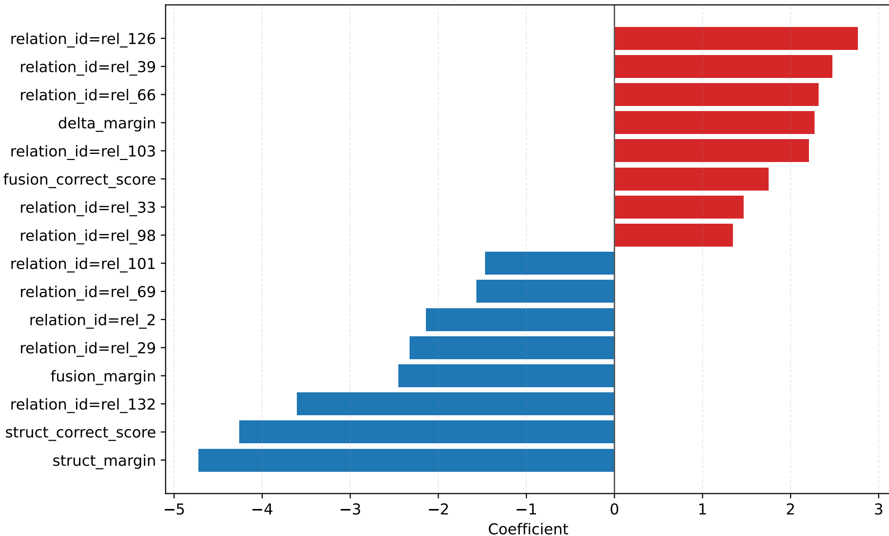
Logistic top coefficients
