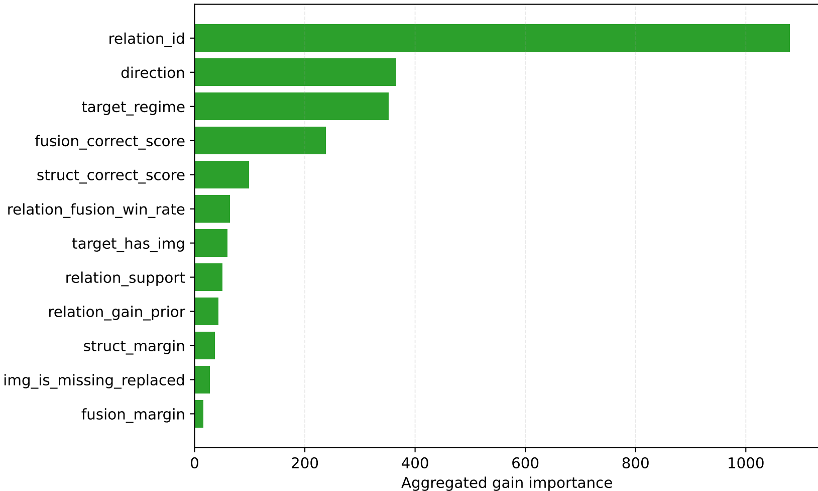
Grouped XGBoost feature importance
