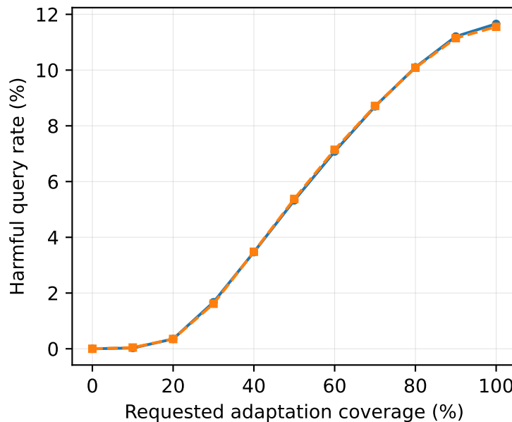
Pooled summary
