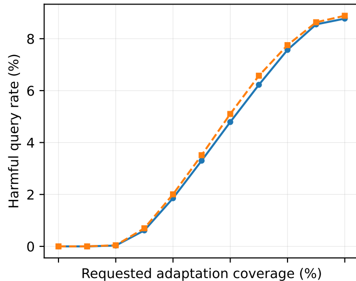
Pooled summary
