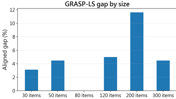
Figure 4: Aligned average GRASP-LS optimality gap by random-instance size, computed only over instances where both MILP and GRASP-LS are feasible.
