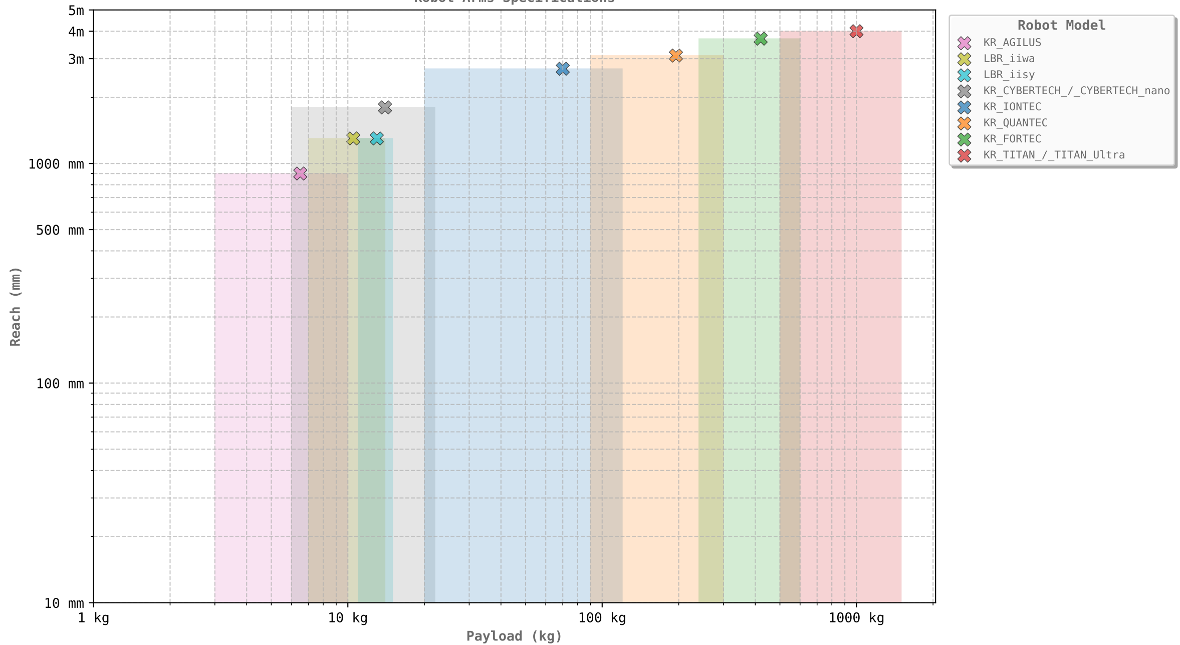
Robot Arms Specifications
