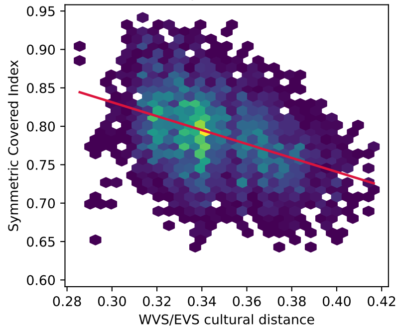
K=200: Spearman r=-0.406
