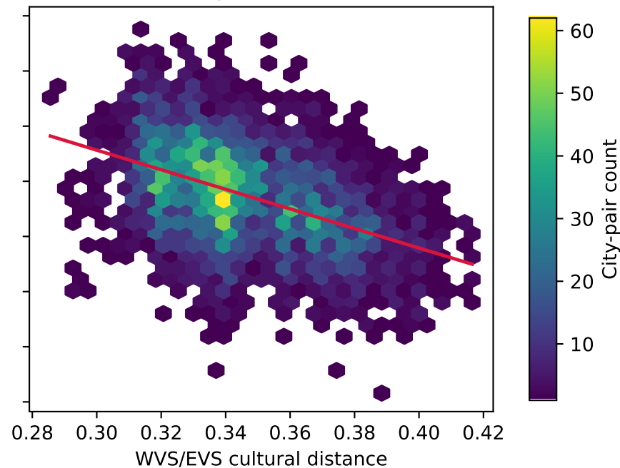
K=1000: Spearman r=-0.443
